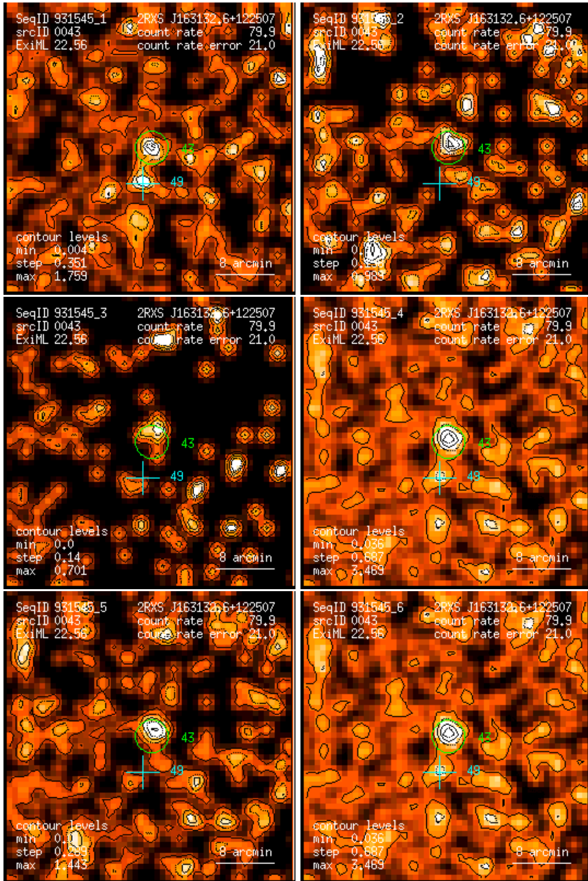
Figure 43: RASS 931545: detection 0043: band rate images, Gaussian filter: (1) PSPC channels 11 – 41, (2) 52 – 90, (3) 91 – 201, (4) 11 – 235, (5) 52 – 201, (6) 11 – 201. Broad band rates in counts/ks. Band rate contour levels in counts/ks/arcmin 2 .
