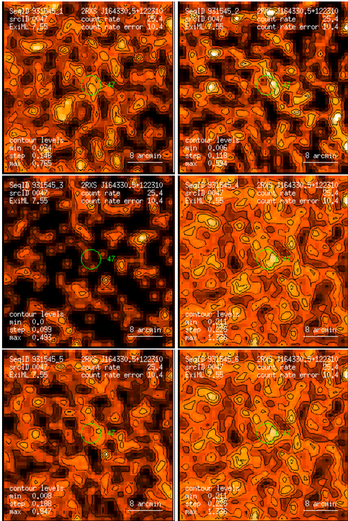
Figure 47: RASS 931545: detection 0047: band rate images, Gaussian filter: (1) PSPC channels 11 – 41, (2) 52 – 90, (3) 91 – 201, (4) 11 – 235, (5) 52 – 201, (6) 11 – 201. Broad band rates in counts/ks. Band rate contour levels in counts/ks/arcmin 2 .
