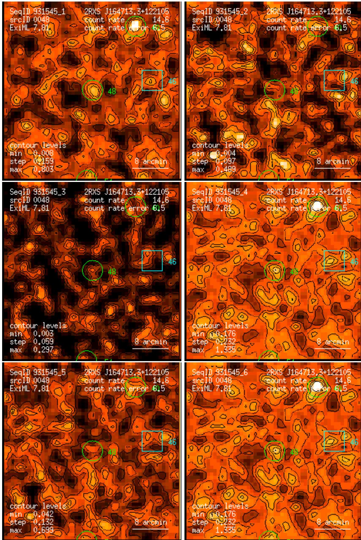
Figure 48: RASS 931545: detection 0048: band rate images, Gaussian filter: (1) PSPC channels 11 – 41, (2) 52 – 90, (3) 91 – 201, (4) 11 – 235, (5) 52 – 201, (6) 11 – 201. Broad band rates in counts/ks. Band rate contour levels in counts/ks/arcmin 2 .
