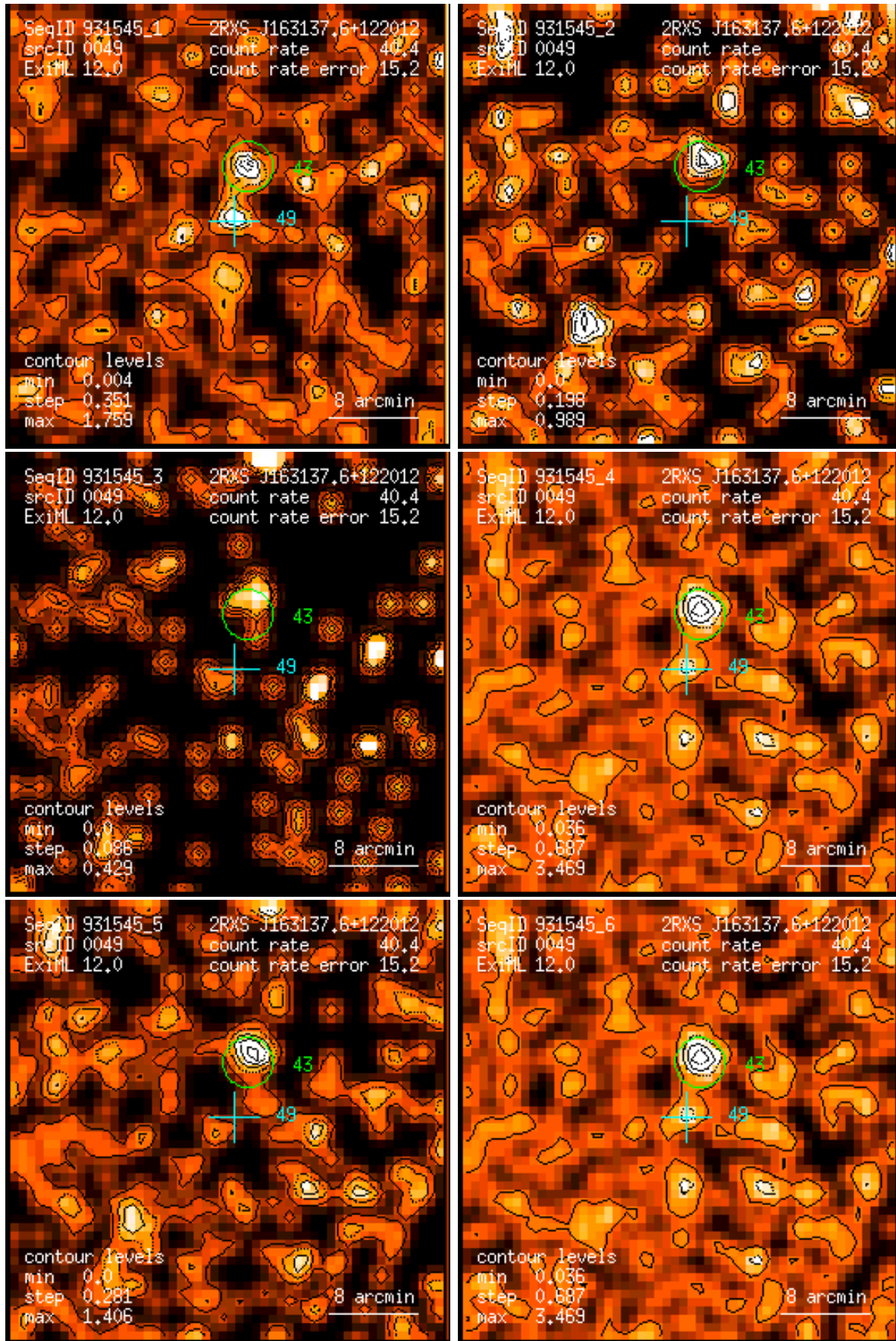
Figure 49: RASS 931545: detection 0049: band rate images, Gaussian filter: (1) PSPC channels 11 – 41, (2) 52 – 90, (3) 91 – 201, (4) 11 – 235, (5) 52 – 201, (6) 11 – 201. Broad band rates in counts/ks. Band rate contour levels in counts/ks/arcmin 2 .
