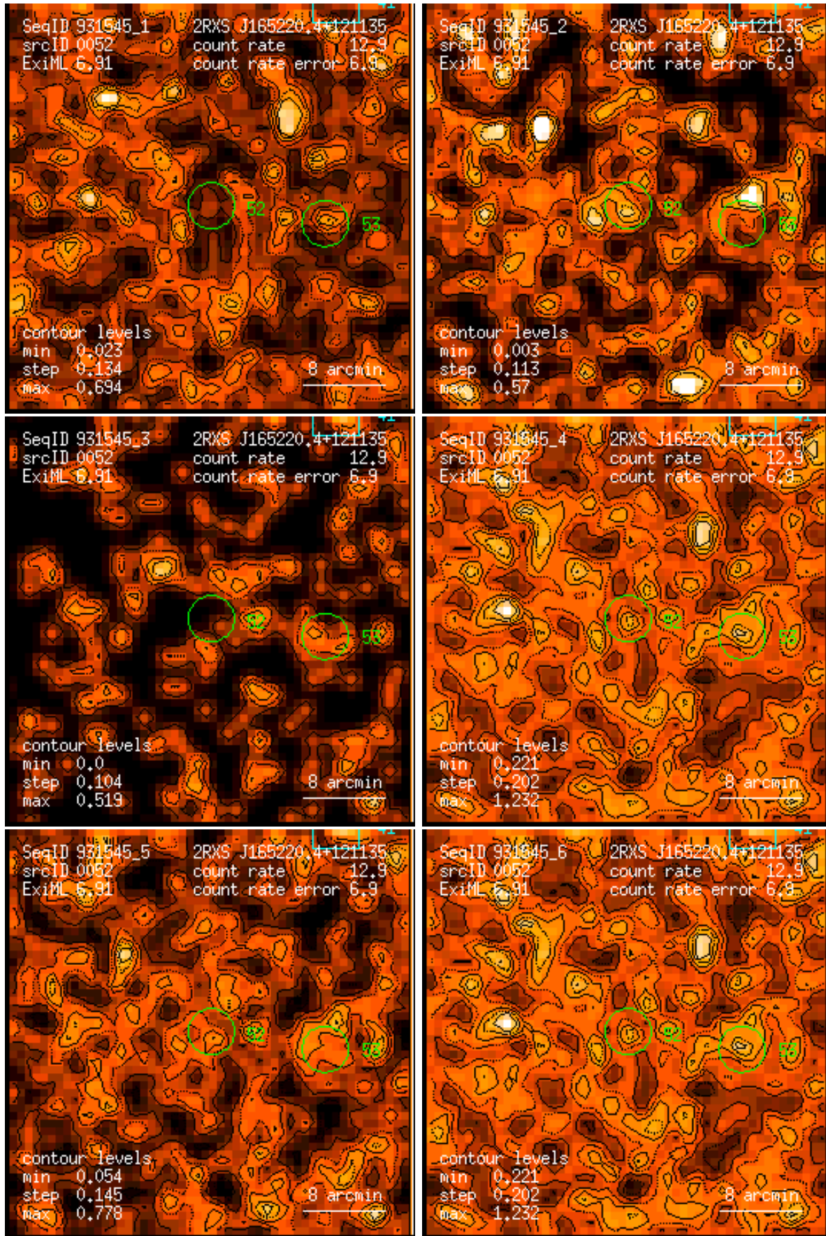
Figure 52: RASS 931545: detection 0052: band rate images, Gaussian filter: (1) PSPC channels 11 – 41, (2) 52 – 90, (3) 91 – 201, (4) 11 – 235, (5) 52 – 201, (6) 11 – 201. Broad band rates in counts/ks. Band rate contour levels in counts/ks/arcmin 2 .
