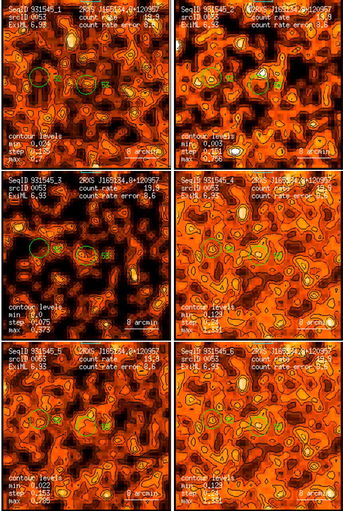
Figure 53: RASS 931545: detection 0053: band rate images, Gaussian filter: (1) PSPC channels 11 – 41, (2) 52 – 90, (3) 91 – 201, (4) 11 – 235, (5) 52 – 201, (6) 11 – 201. Broad band rates in counts/ks. Band rate contour levels in counts/ks/arcmin 2 .
