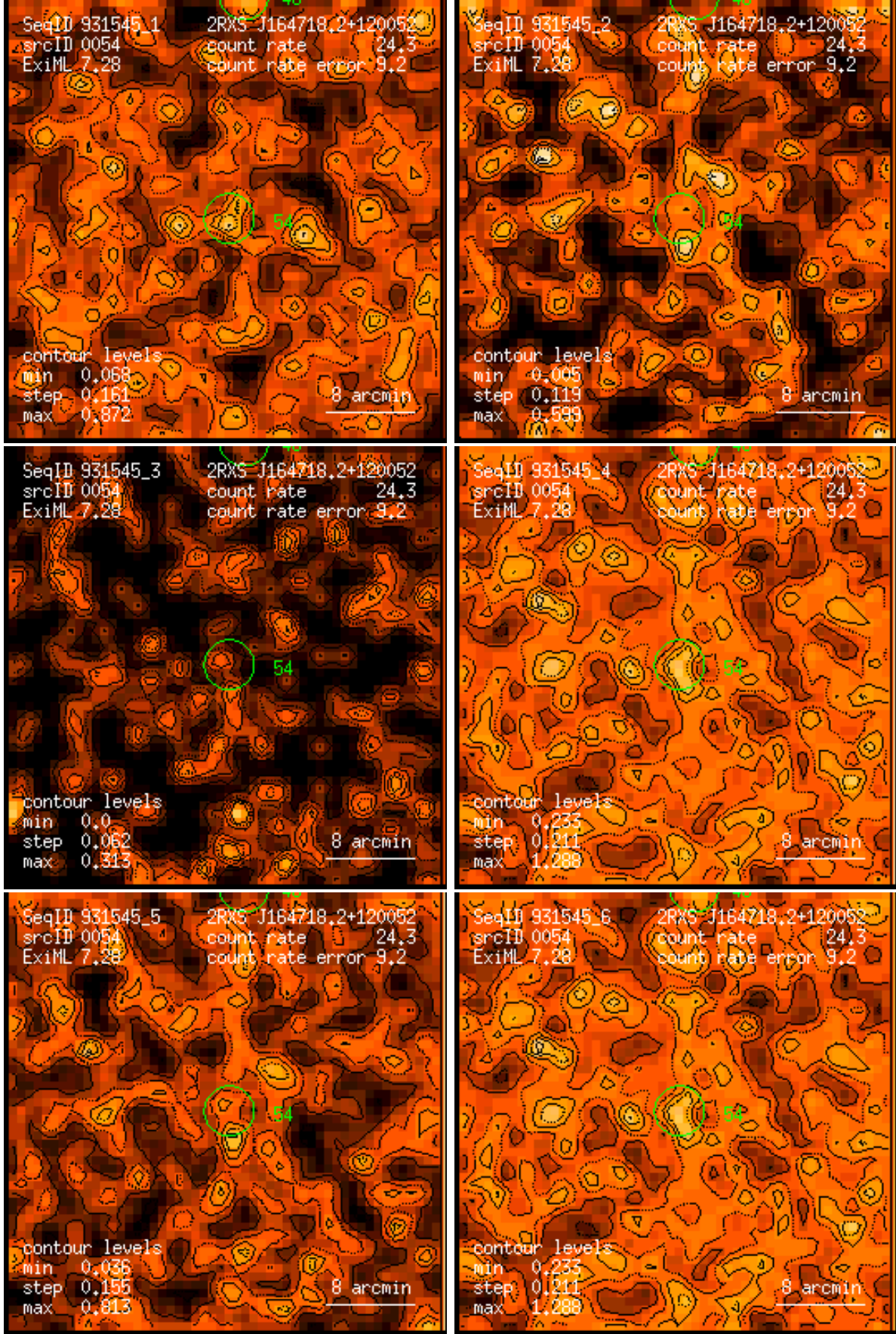
Figure 54: RASS 931545: detection 0054: band rate images, Gaussian filter: (1) PSPC channels 11 – 41, (2) 52 – 90, (3) 91 – 201, (4) 11 – 235, (5) 52 – 201, (6) 11 – 201. Broad band rates in counts/ks. Band rate contour levels in counts/ks/arcmin 2 .
