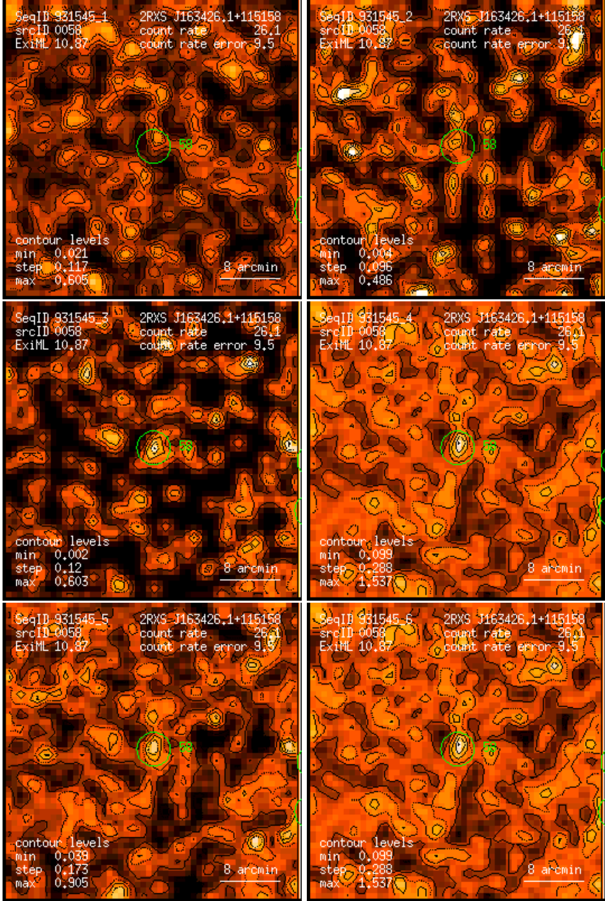
Figure 58: RASS 931545: detection 0058: band rate images, Gaussian filter: (1) PSPC channels 11 – 41, (2) 52 – 90, (3) 91 – 201, (4) 11 – 235, (5) 52 – 201, (6) 11 – 201. Broad band rates in counts/ks. Band rate contour levels in counts/ks/arcmin 2 .
