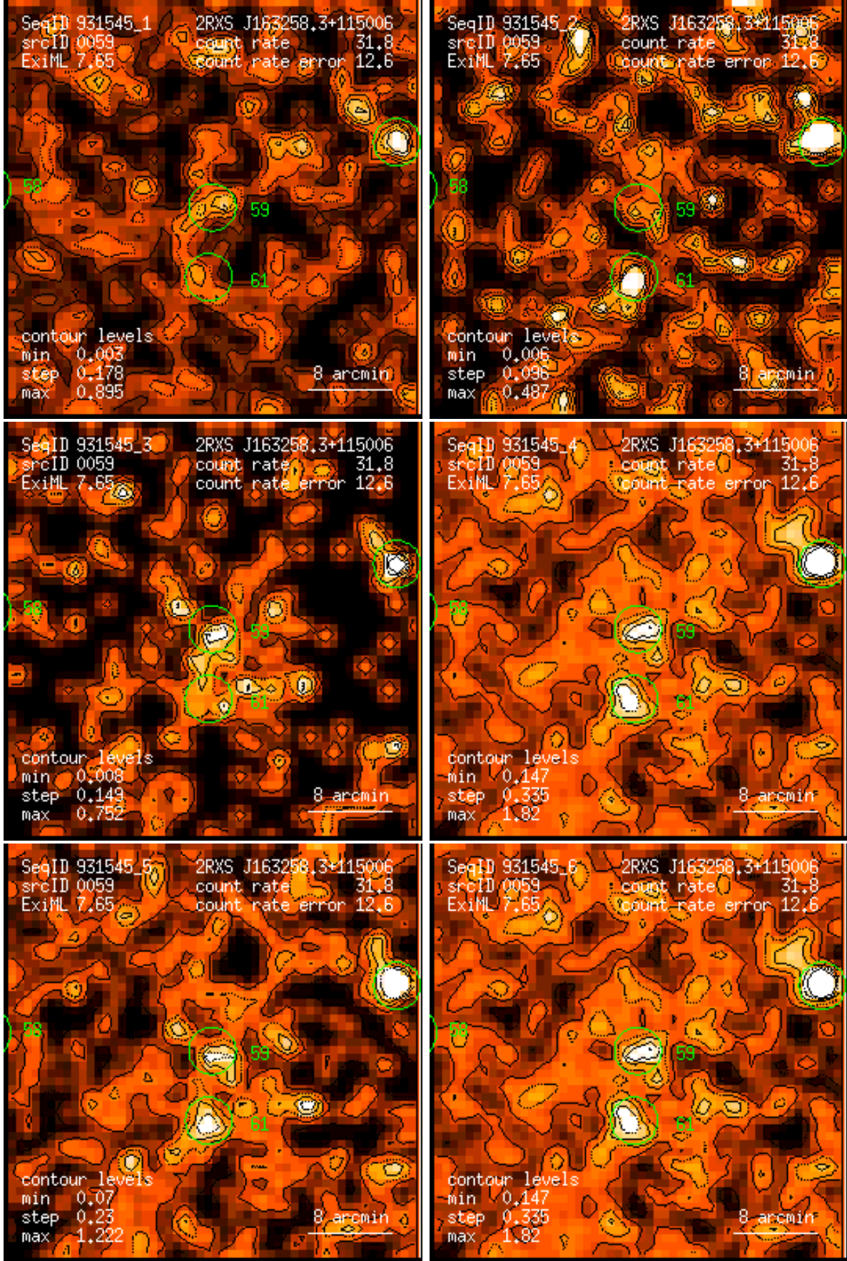
Figure 59: RASS 931545: detection 0059: band rate images, Gaussian filter: (1) PSPC channels 11 – 41, (2) 52 – 90, (3) 91 – 201, (4) 11 – 235, (5) 52 – 201, (6) 11 – 201. Broad band rates in counts/ks. Band rate contour levels in counts/ks/arcmin 2 .
