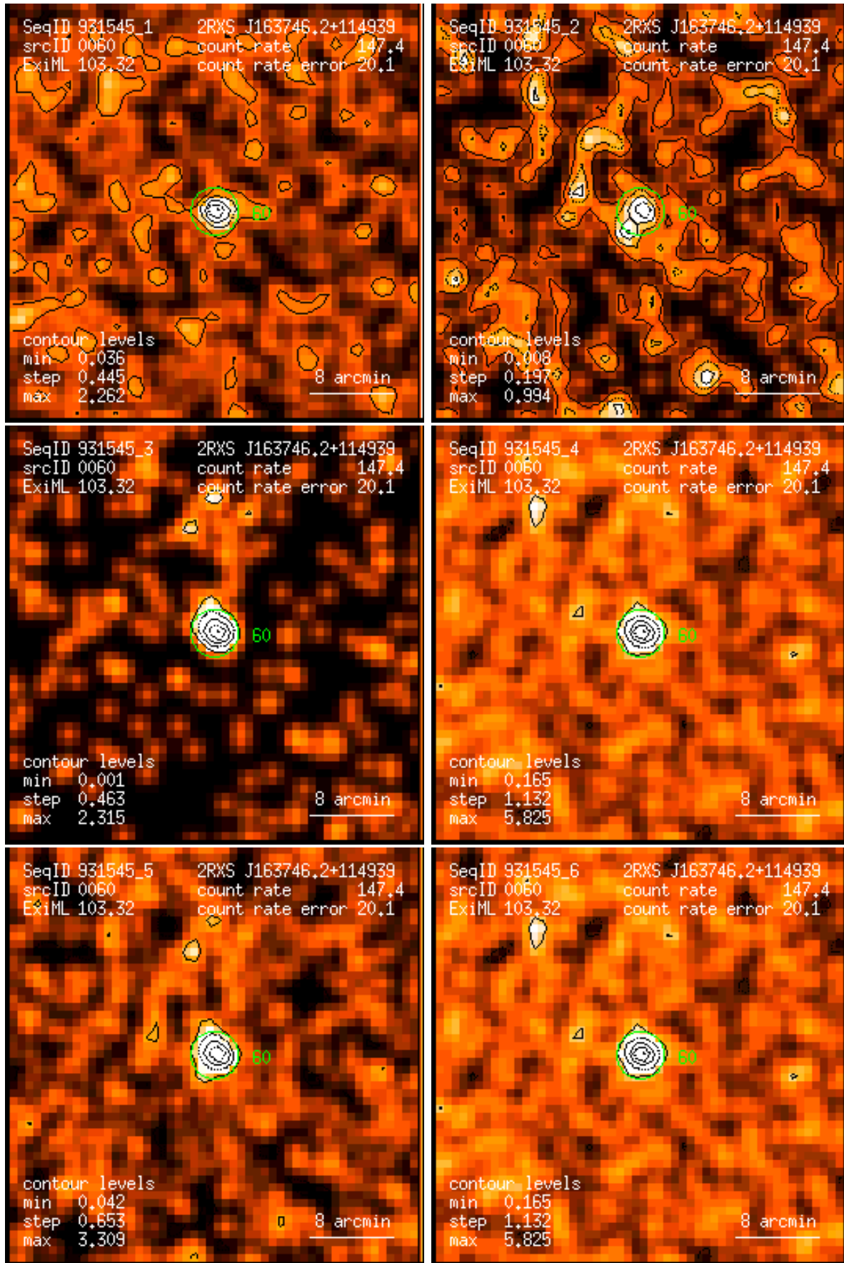
Figure 60: RASS 931545: detection 0060: band rate images, Gaussian filter: (1) PSPC channels 11 – 41, (2) 52 – 90, (3) 91 – 201, (4) 11 – 235, (5) 52 – 201, (6) 11 – 201. Broad band rates in counts/ks. Band rate contour levels in counts/ks/arcmin 2 .
