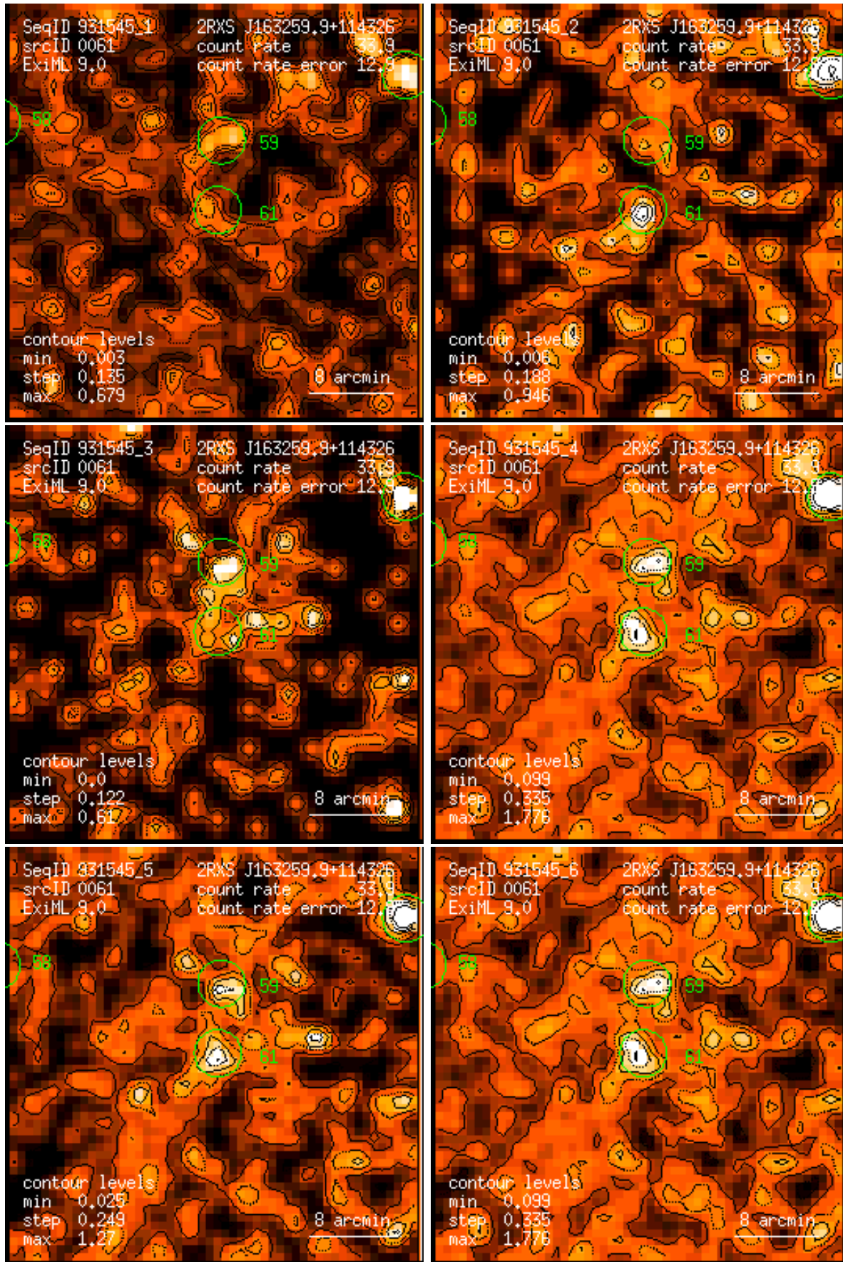
Figure 61: RASS 931545: detection 0061: band rate images, Gaussian filter: (1) PSPC channels 11 – 41, (2) 52 – 90, (3) 91 – 201, (4) 11 – 235, (5) 52 – 201, (6) 11 – 201. Broad band rates in counts/ks. Band rate contour levels in counts/ks/arcmin 2 .
