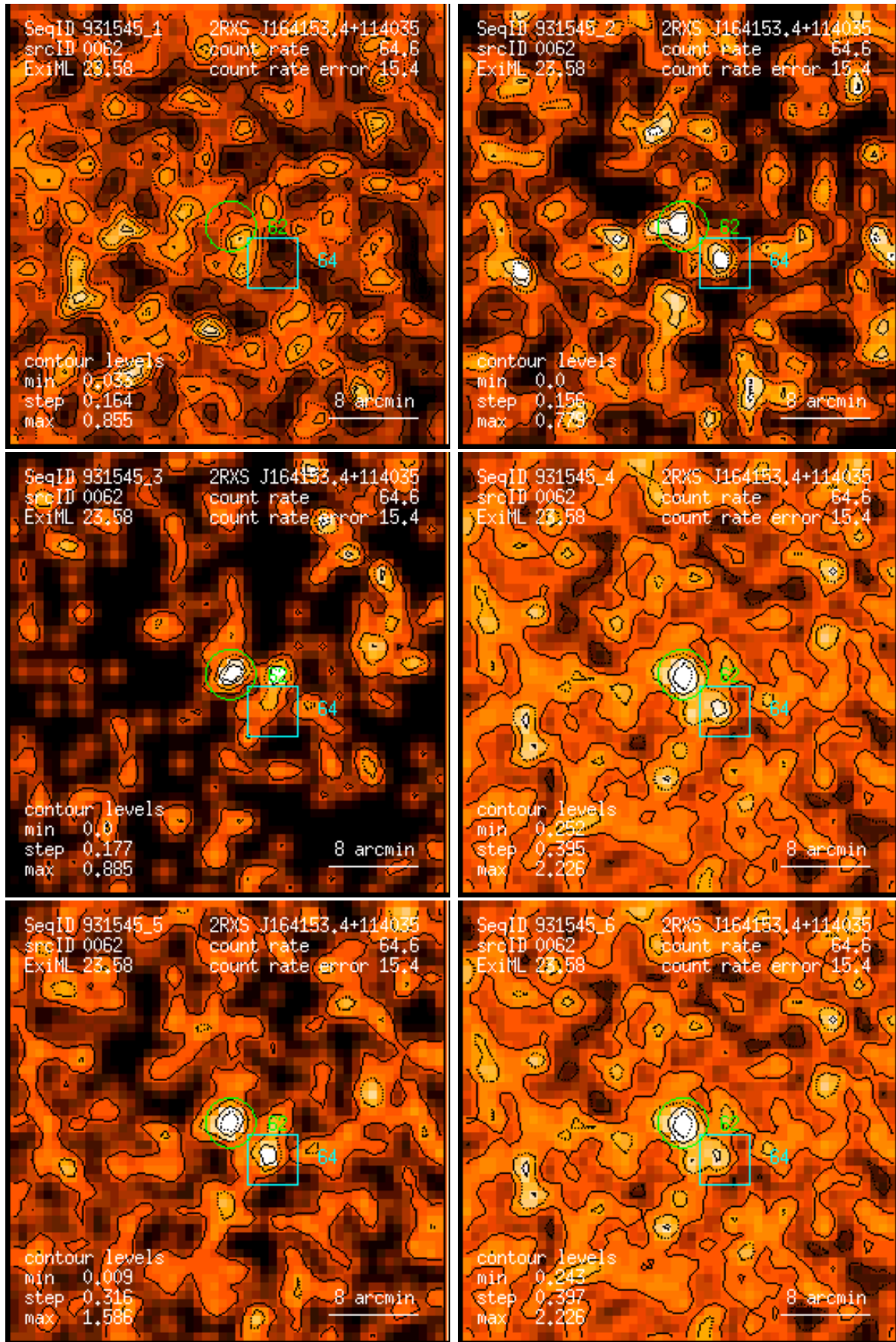
Figure 62: RASS 931545: detection 0062: band rate images, Gaussian filter: (1) PSPC channels 11 – 41, (2) 52 – 90, (3) 91 – 201, (4) 11 – 235, (5) 52 – 201, (6) 11 – 201. Broad band rates in counts/ks. Band rate contour levels in counts/ks/arcmin 2 .
