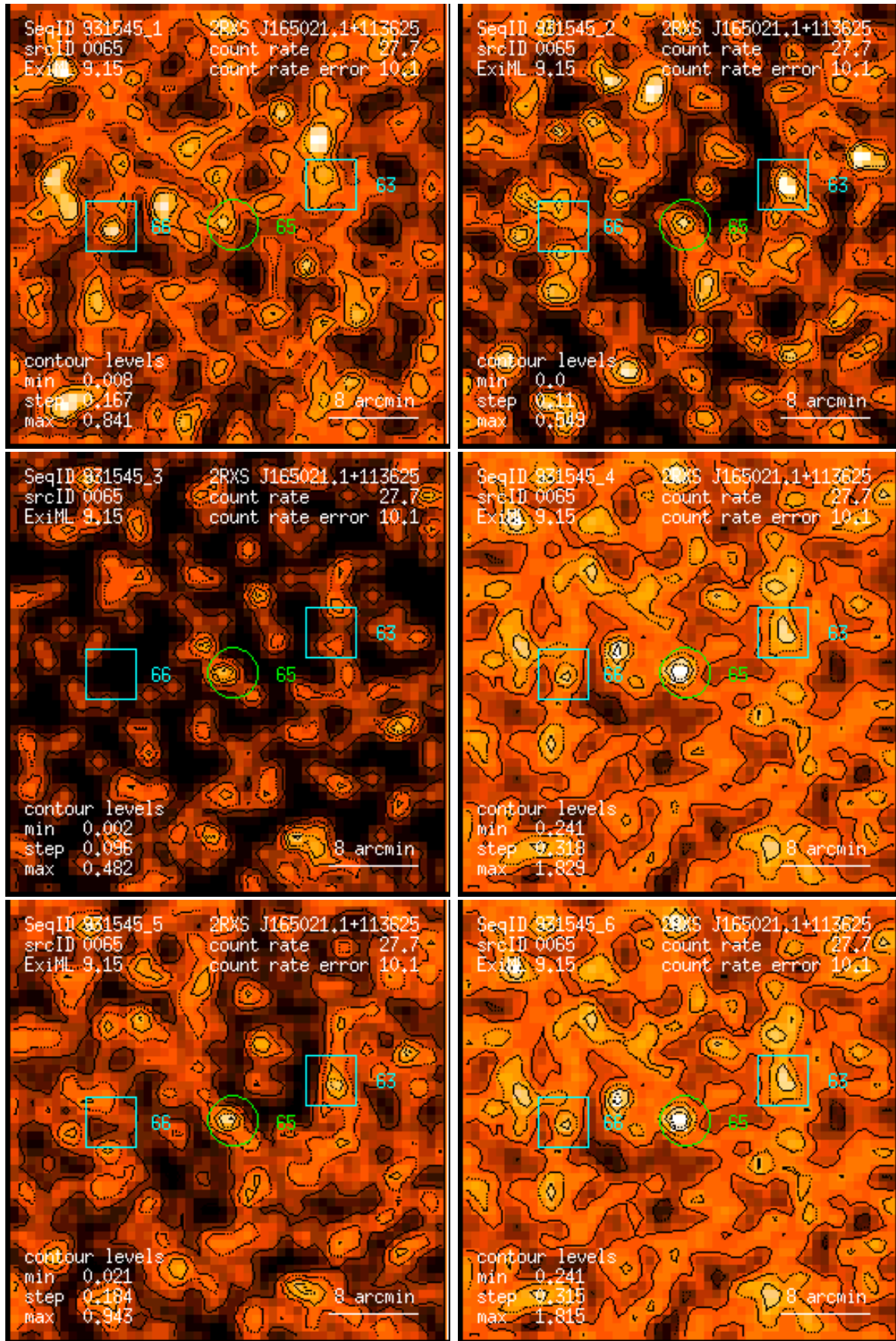
Figure 65: RASS 931545: detection 0065: band rate images, Gaussian filter: (1) PSPC channels 11 – 41, (2) 52 – 90, (3) 91 – 201, (4) 11 – 235, (5) 52 – 201, (6) 11 – 201. Broad band rates in counts/ks. Band rate contour levels in counts/ks/arcmin 2 .
