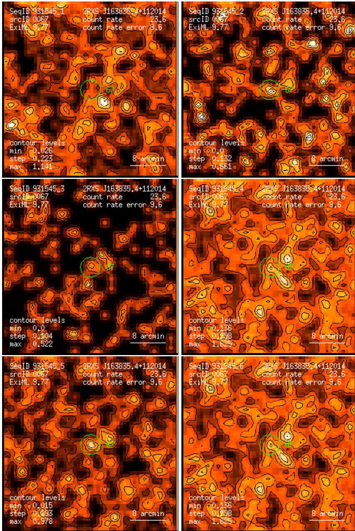
Figure 67: RASS 931545: detection 0067: band rate images, Gaussian filter: (1) PSPC channels 11 – 41, (2) 52 – 90, (3) 91 – 201, (4) 11 – 235, (5) 52 – 201, (6) 11 – 201. Broad band rates in counts/ks. Band rate contour levels in counts/ks/arcmin 2 .
