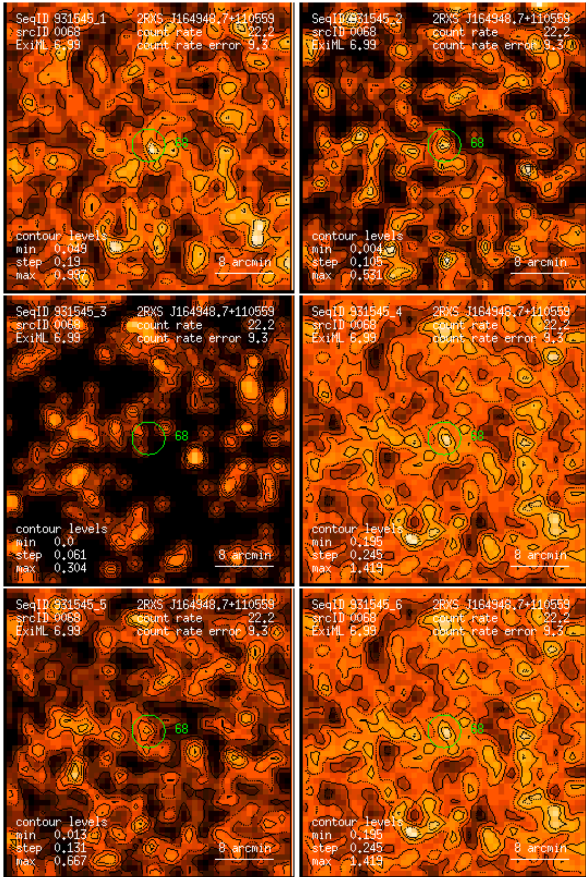
Figure 68: RASS 931545: detection 0068: band rate images, Gaussian filter: (1) PSPC channels 11 – 41, (2) 52 – 90, (3) 91 – 201, (4) 11 – 235, (5) 52 – 201, (6) 11 – 201. Broad band rates in counts/ks. Band rate contour levels in counts/ks/arcmin 2 .
