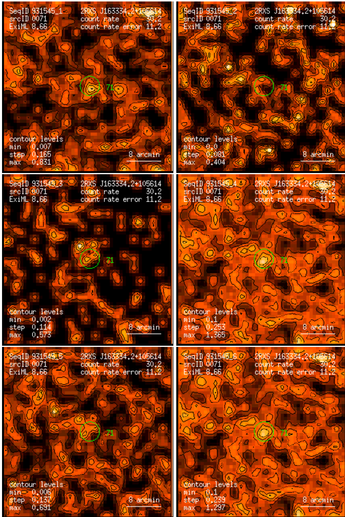
Figure 71: RASS 931545: detection 0071: band rate images, Gaussian filter: (1) PSPC channels 11 – 41, (2) 52 – 90, (3) 91 – 201, (4) 11 – 235, (5) 52 – 201, (6) 11 – 201. Broad band rates in counts/ks. Band rate contour levels in counts/ks/arcmin 2 .
