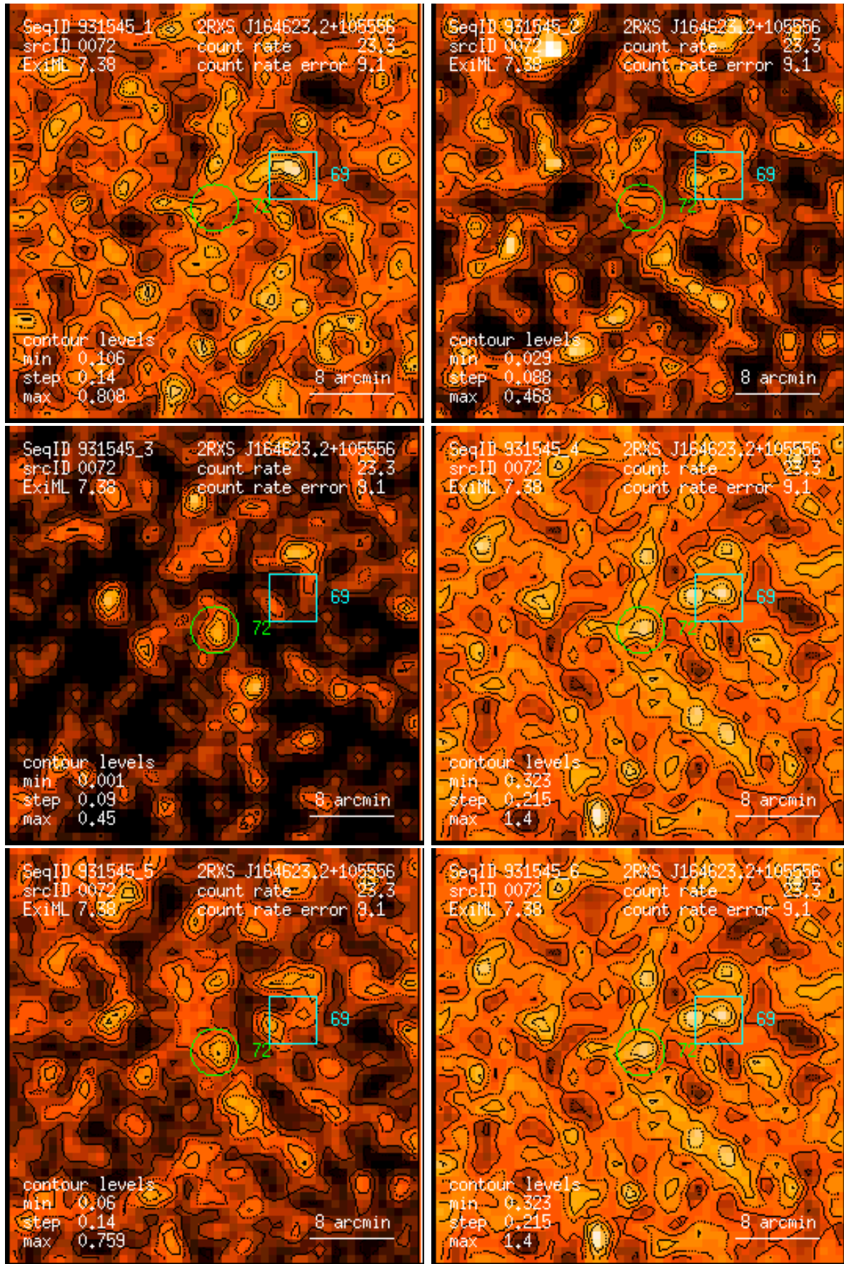
Figure 72: RASS 931545: detection 0072: band rate images, Gaussian filter: (1) PSPC channels 11 – 41, (2) 52 – 90, (3) 91 – 201, (4) 11 – 235, (5) 52 – 201, (6) 11 – 201. Broad band rates in counts/ks. Band rate contour levels in counts/ks/arcmin 2 .
