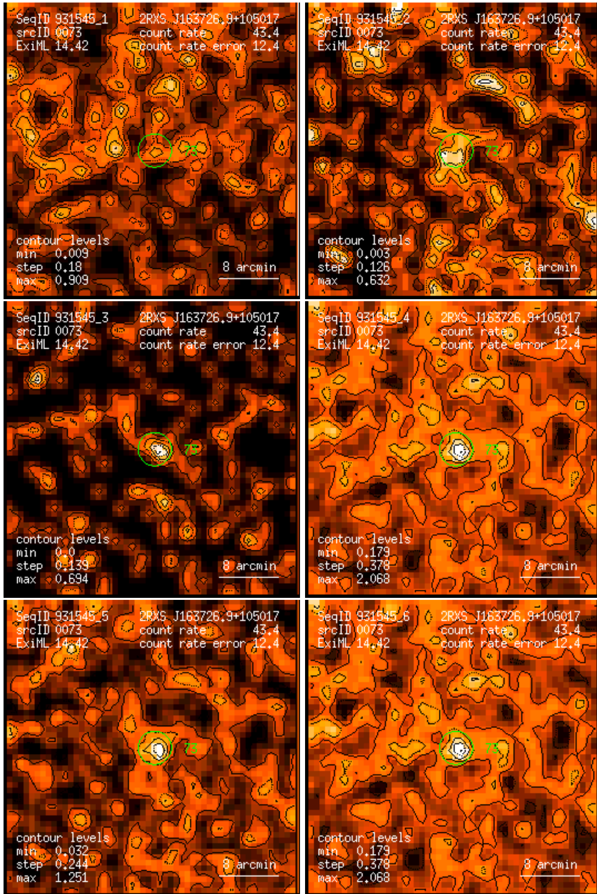
Figure 73: RASS 931545: detection 0073: band rate images, Gaussian filter: (1) PSPC channels 11 – 41, (2) 52 – 90, (3) 91 – 201, (4) 11 – 235, (5) 52 – 201, (6) 11 – 201. Broad band rates in counts/ks. Band rate contour levels in counts/ks/arcmin 2 .
