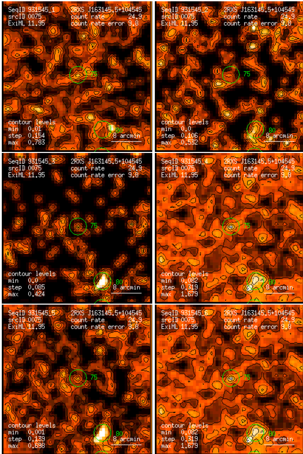
Figure 75: RASS 931545: detection 0075: band rate images, Gaussian filter: (1) PSPC channels 11 – 41, (2) 52 – 90, (3) 91 – 201, (4) 11 – 235, (5) 52 – 201, (6) 11 – 201. Broad band rates in counts/ks. Band rate contour levels in counts/ks/arcmin 2 .
