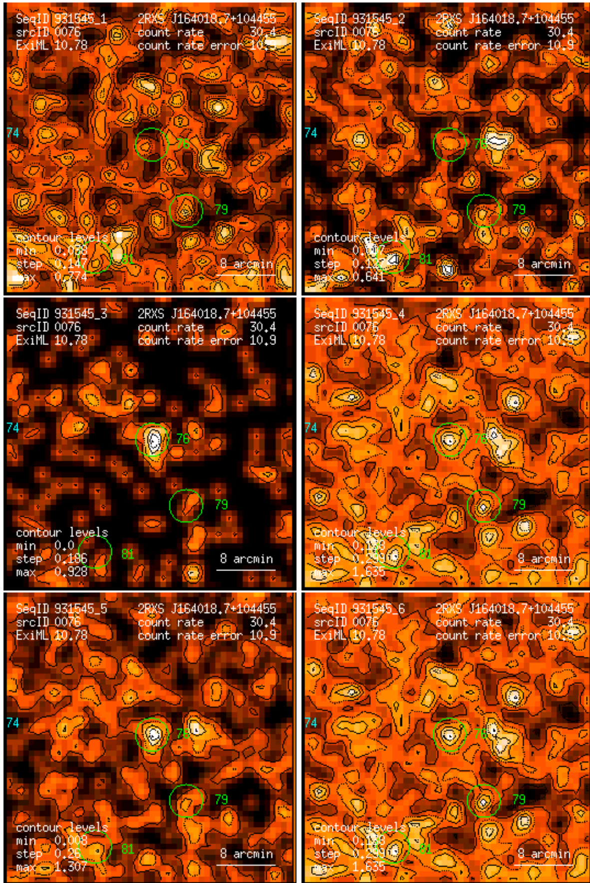
Figure 76: RASS 931545: detection 0076: band rate images, Gaussian filter: (1) PSPC channels 11 – 41, (2) 52 – 90, (3) 91 – 201, (4) 11 – 235, (5) 52 – 201, (6) 11 – 201. Broad band rates in counts/ks. Band rate contour levels in counts/ks/arcmin 2 .
