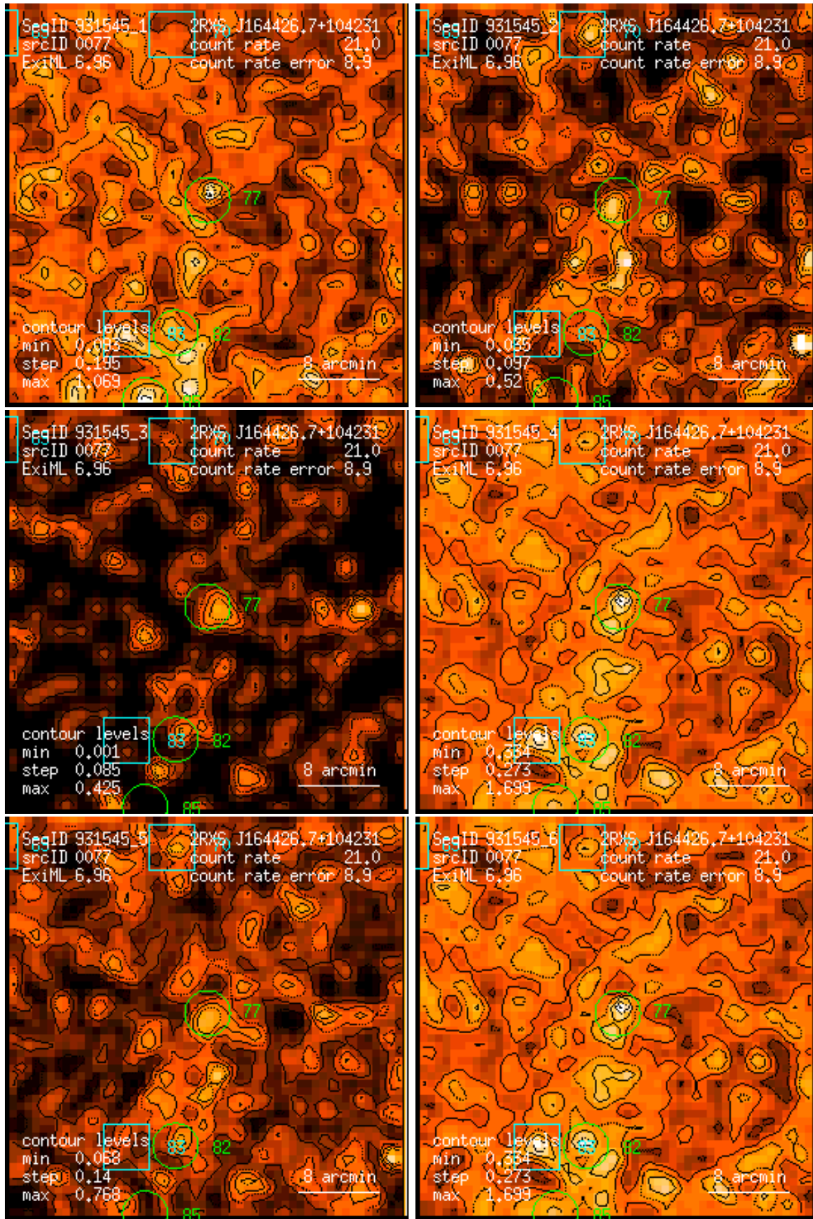
Figure 77: RASS 931545: detection 0077: band rate images, Gaussian filter: (1) PSPC channels 11 – 41, (2) 52 – 90, (3) 91 – 201, (4) 11 – 235, (5) 52 – 201, (6) 11 – 201. Broad band rates in counts/ks. Band rate contour levels in counts/ks/arcmin 2 .
