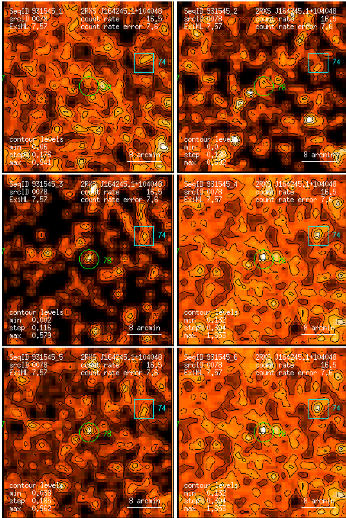
Figure 78: RASS 931545: detection 0078: band rate images, Gaussian filter: (1) PSPC channels 11 – 41, (2) 52 – 90, (3) 91 – 201, (4) 11 – 235, (5) 52 – 201, (6) 11 – 201. Broad band rates in counts/ks. Band rate contour levels in counts/ks/arcmin 2 .
