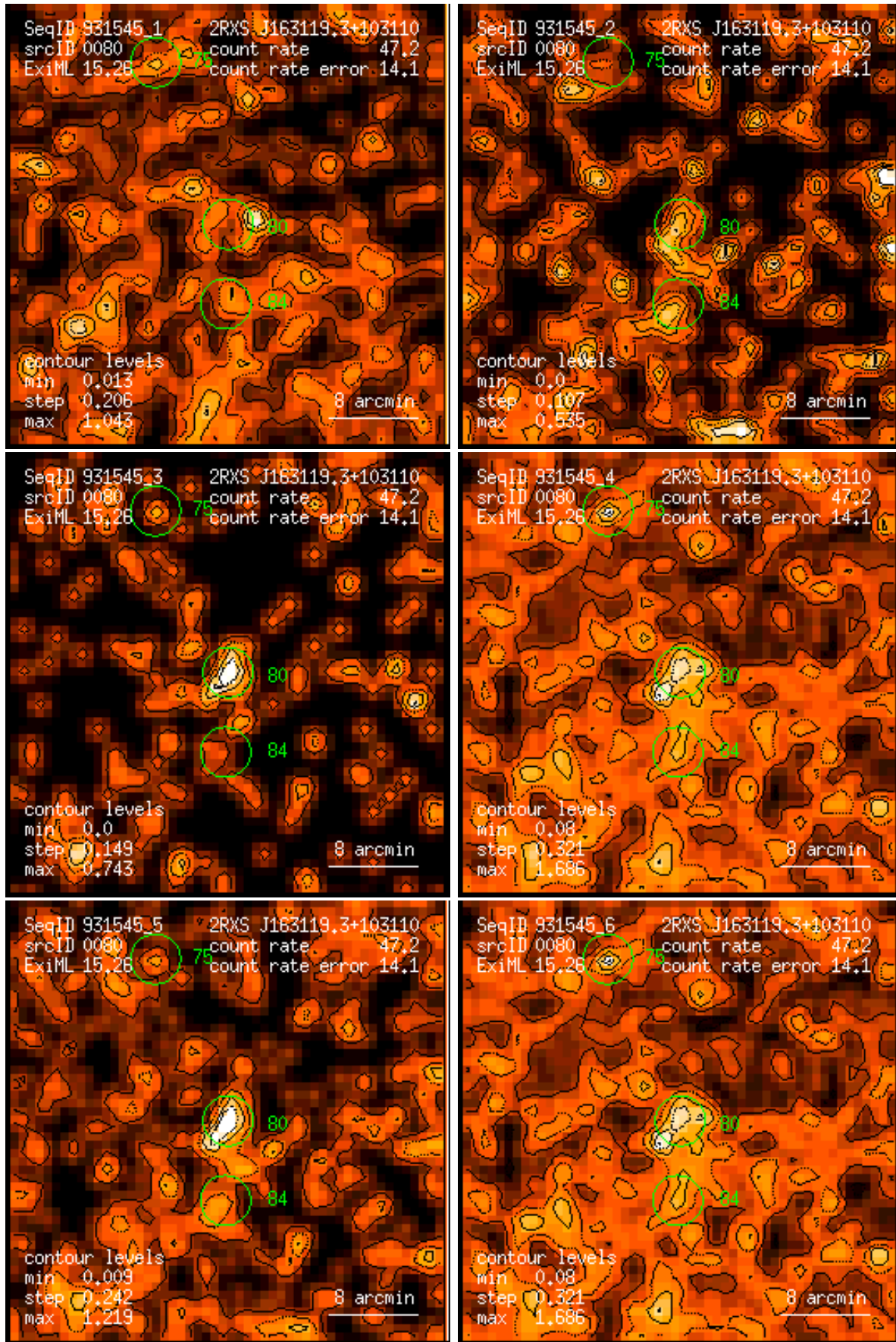
Figure 80: RASS 931545: detection 0080: band rate images, Gaussian filter: (1) PSPC channels 11 – 41, (2) 52 – 90, (3) 91 – 201, (4) 11 – 235, (5) 52 – 201, (6) 11 – 201. Broad band rates in counts/ks. Band rate contour levels in counts/ks/arcmin 2 .
