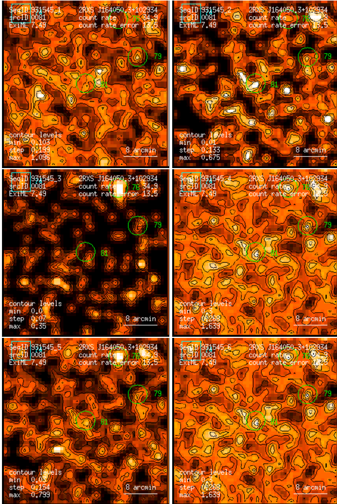
Figure 81: RASS 931545: detection 0081: band rate images, Gaussian filter: (1) PSPC channels 11 – 41, (2) 52 – 90, (3) 91 – 201, (4) 11 – 235, (5) 52 – 201, (6) 11 – 201. Broad band rates in counts/ks. Band rate contour levels in counts/ks/arcmin 2 .
