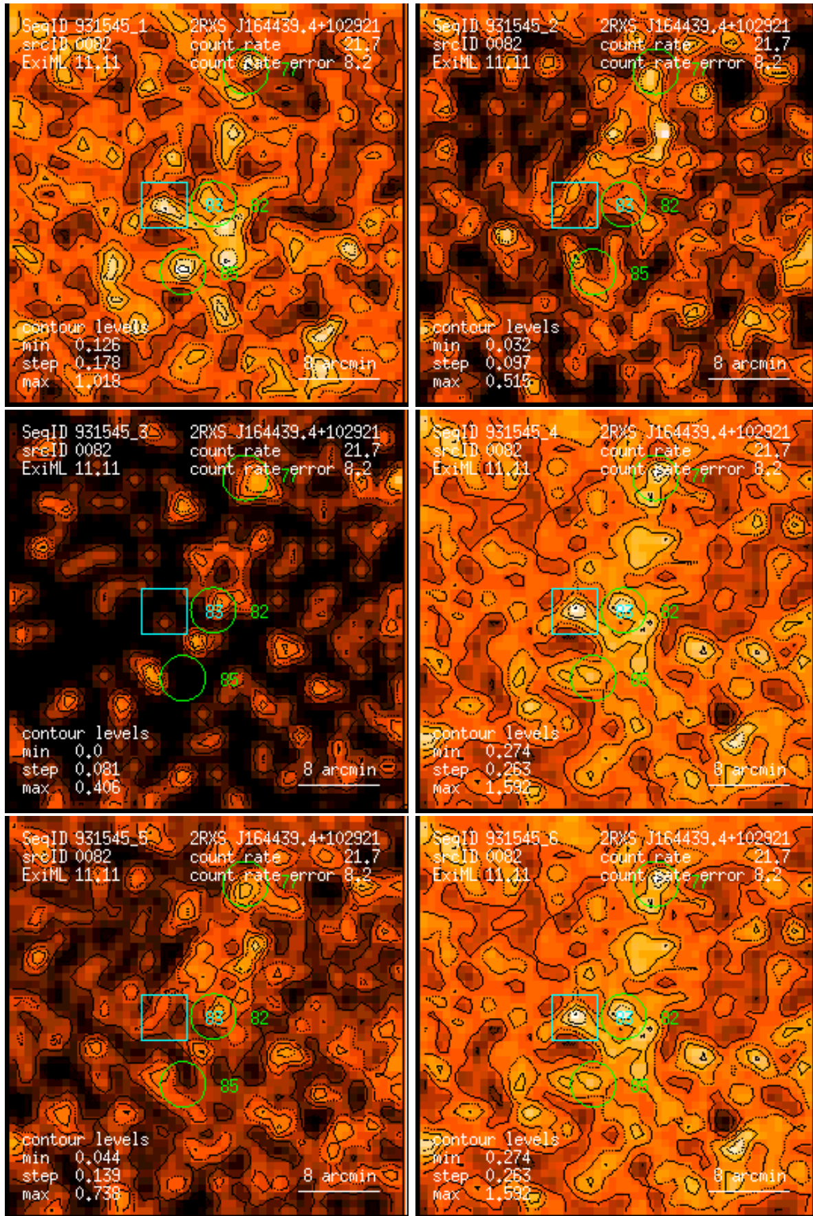
Figure 82: RASS 931545: detection 0082: band rate images, Gaussian filter: (1) PSPC channels 11 – 41, (2) 52 – 90, (3) 91 – 201, (4) 11 – 235, (5) 52 – 201, (6) 11 – 201. Broad band rates in counts/ks. Band rate contour levels in counts/ks/arcmin 2 .
