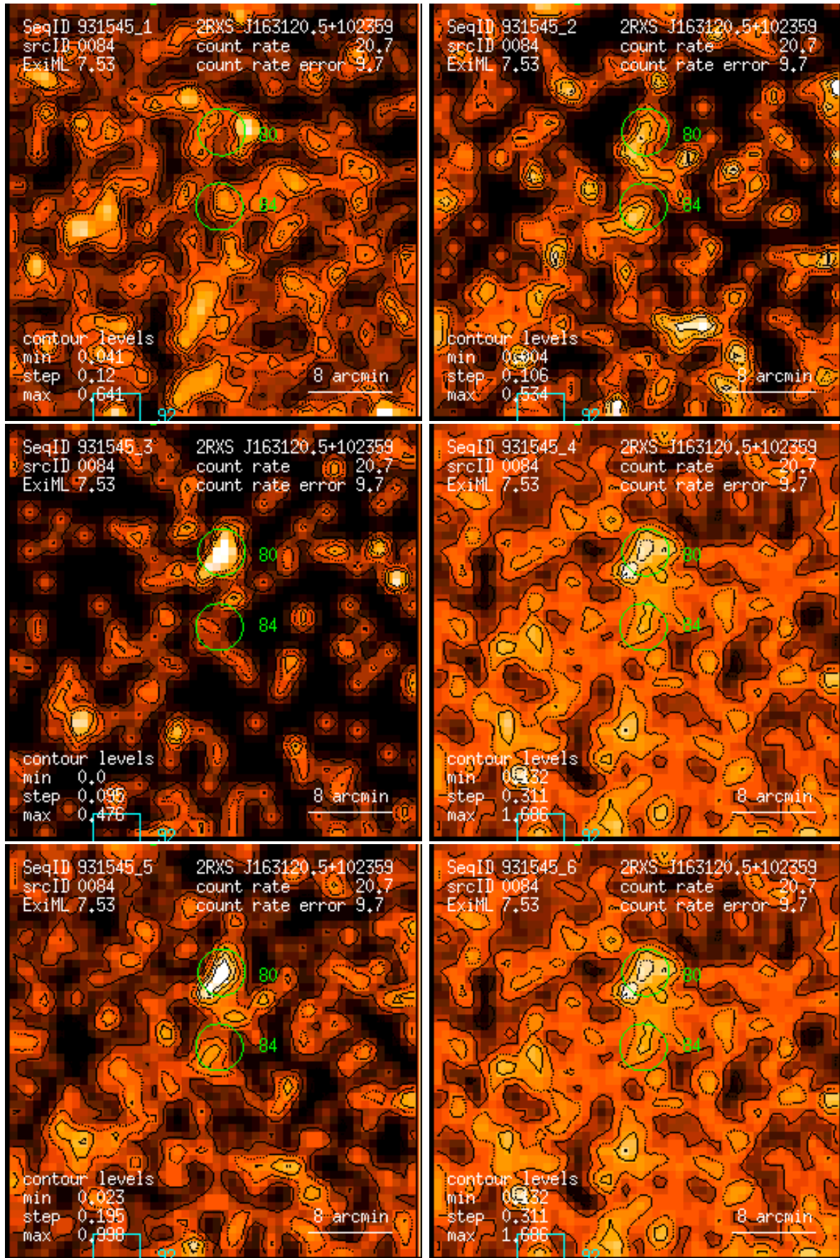
Figure 84: RASS 931545: detection 0084: band rate images, Gaussian filter: (1) PSPC channels 11 – 41, (2) 52 – 90, (3) 91 – 201, (4) 11 – 235, (5) 52 – 201, (6) 11 – 201. Broad band rates in counts/ks. Band rate contour levels in counts/ks/arcmin 2 .
