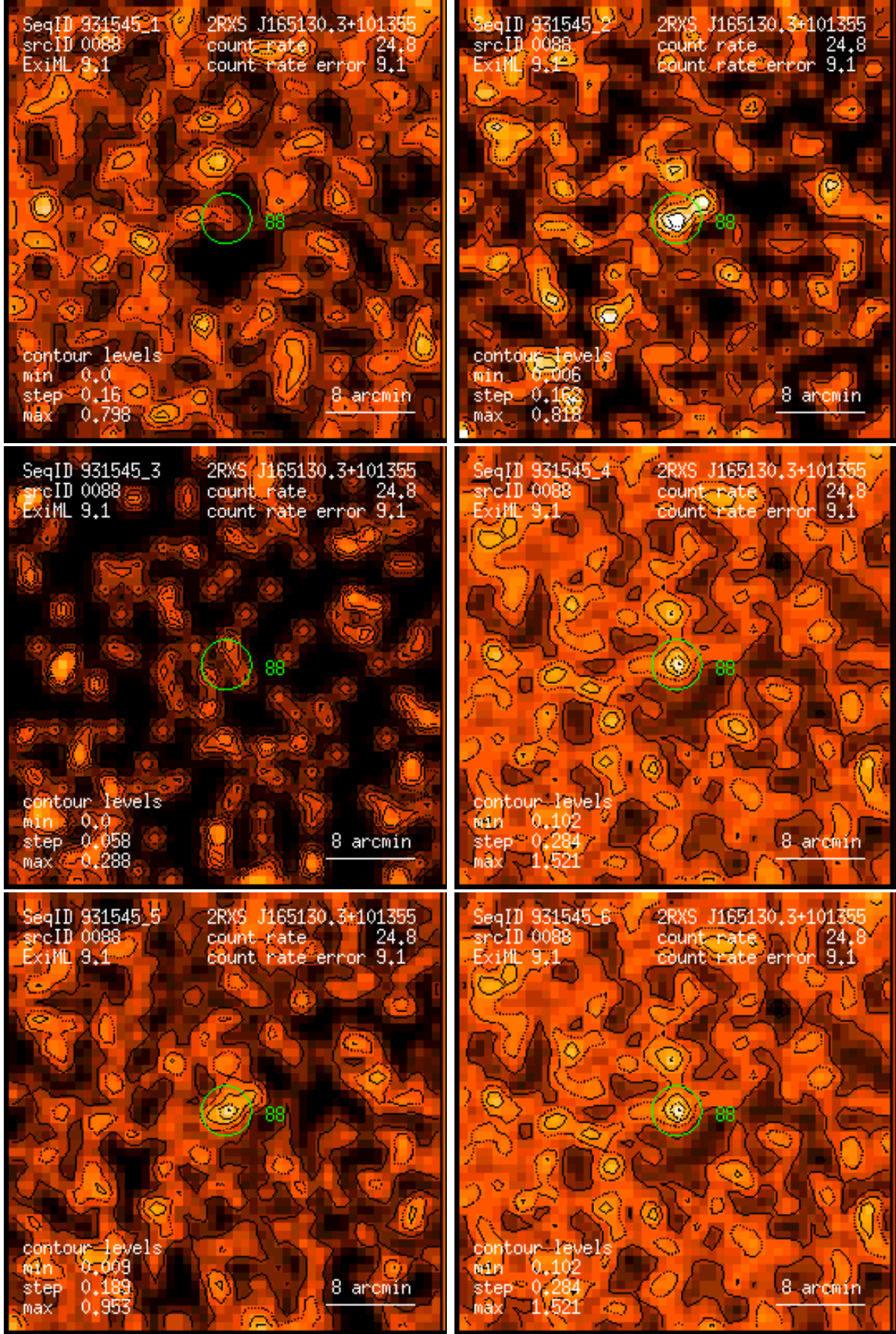
Figure 88: RASS 931545: detection 0088: band rate images, Gaussian filter: (1) PSPC channels 11 – 41, (2) 52 – 90, (3) 91 – 201, (4) 11 – 235, (5) 52 – 201, (6) 11 – 201. Broad band rates in counts/ks. Band rate contour levels in counts/ks/arcmin 2 .
