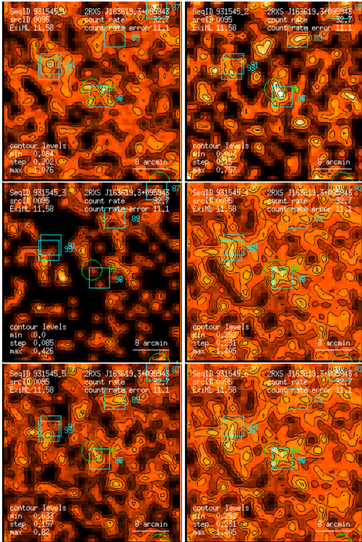
Figure 95: RASS 931545: detection 0095: band rate images, Gaussian filter: (1) PSPC channels 11 – 41, (2) 52 – 90, (3) 91 – 201, (4) 11 – 235, (5) 52 – 201, (6) 11 – 201. Broad band rates in counts/ks. Band rate contour levels in counts/ks/arcmin 2 .
