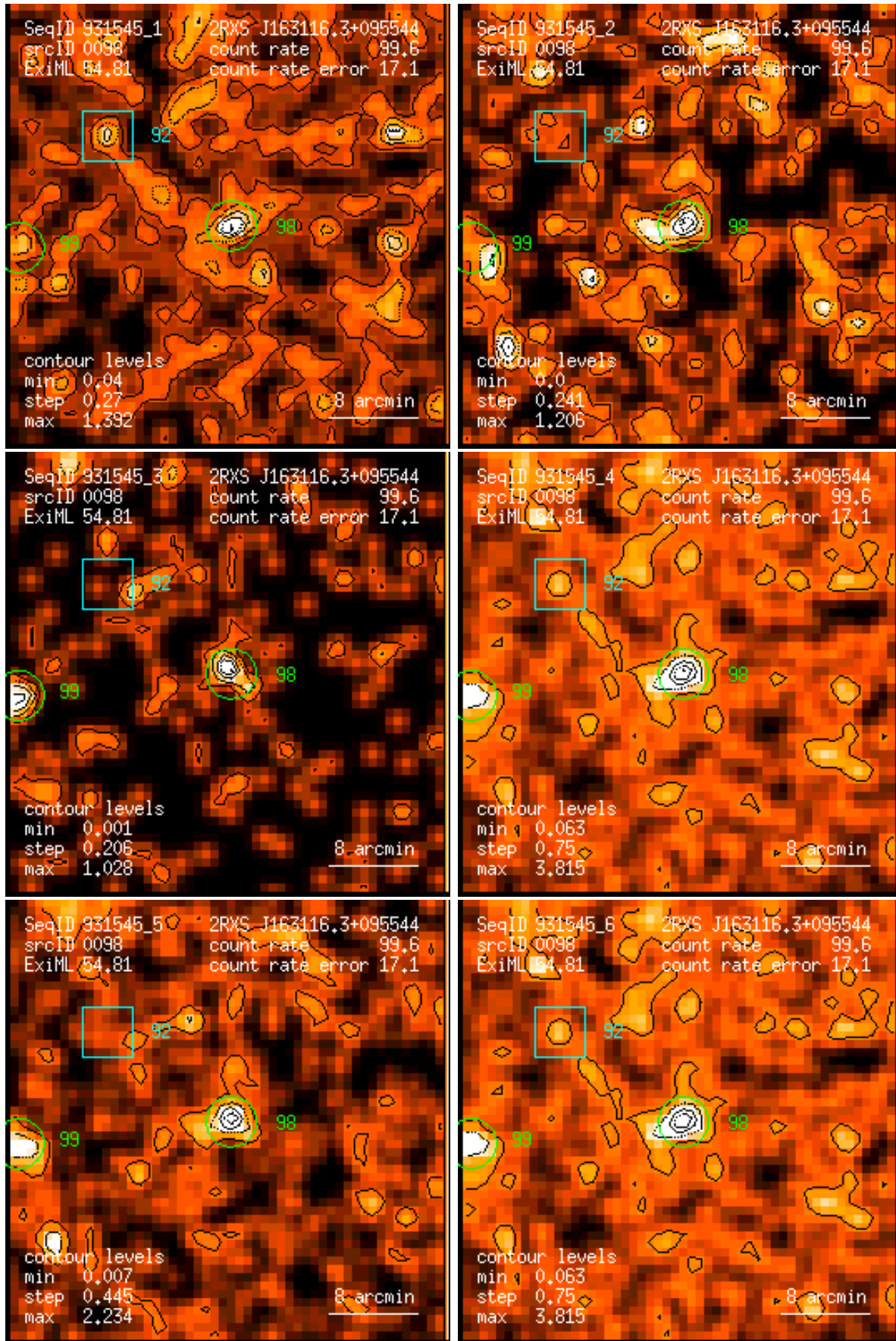
Figure 98: RASS 931545: detection 0098: band rate images, Gaussian filter: (1) PSPC channels 11 – 41, (2) 52 – 90, (3) 91 – 201, (4) 11 – 235, (5) 52 – 201, (6) 11 – 201. Broad band rates in counts/ks. Band rate contour levels in counts/ks/arcmin 2 .
