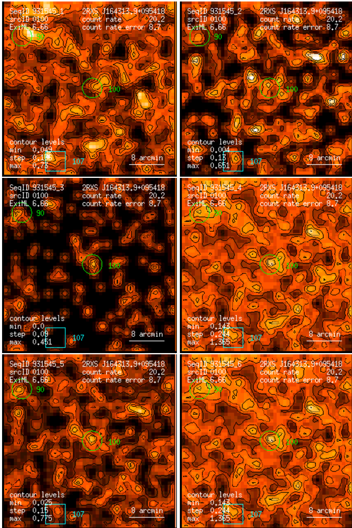
Figure 100: RASS 931545: detection 0100: band rate images, Gaussian filter: (1) PSPC channels 11 – 41, (2) 52 – 90, (3) 91 – 201, (4) 11 – 235, (5) 52 – 201, (6) 11 – 201. Broad band rates in counts/ks. Band rate contour levels in counts/ks/arcmin 2 .
