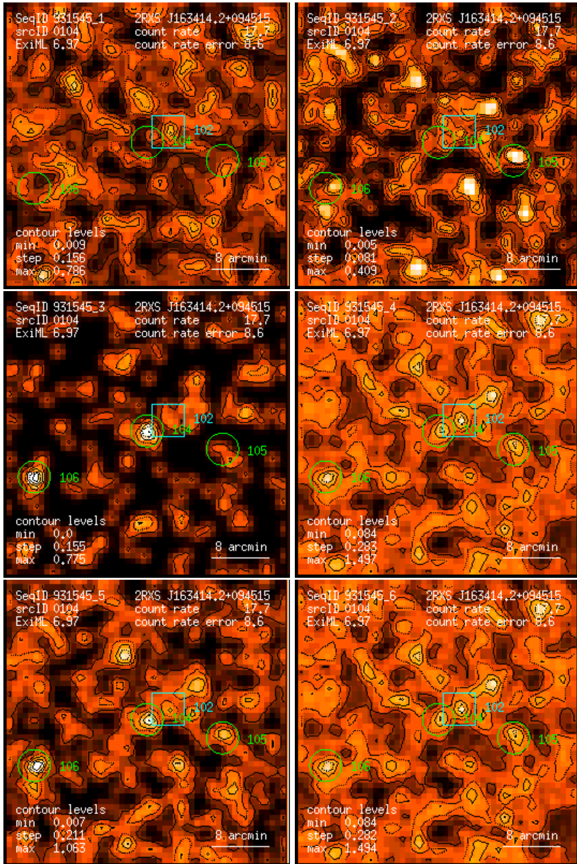
Figure 104: RASS 931545: detection 0104: band rate images, Gaussian filter: (1) PSPC channels 11 – 41, (2) 52 – 90, (3) 91 – 201, (4) 11 – 235, (5) 52 – 201, (6) 11 – 201. Broad band rates in counts/ks. Band rate contour levels in counts/ks/arcmin 2 .
