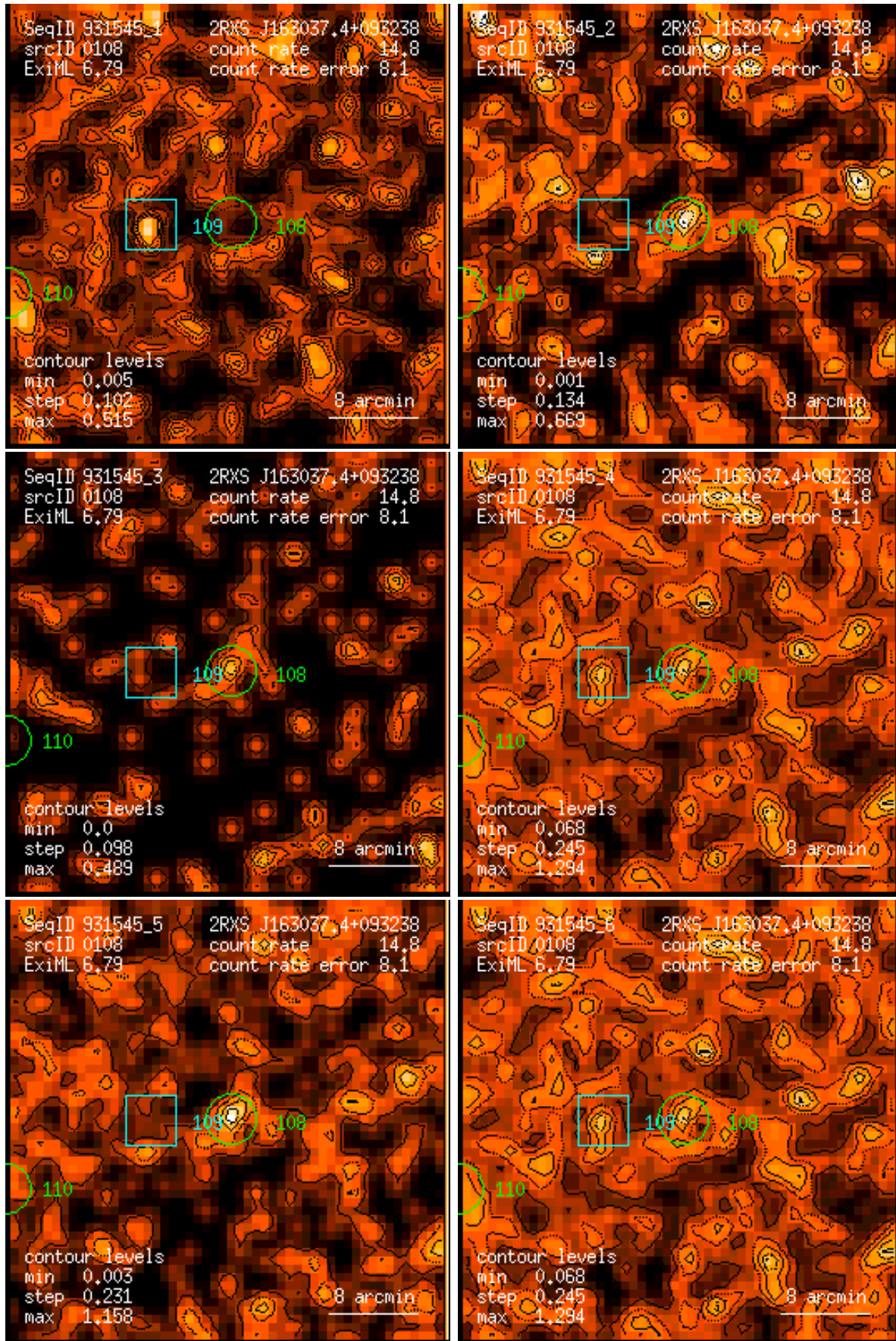
Figure 108: RASS 931545: detection 0108: band rate images, Gaussian filter: (1) PSPC channels 11 – 41, (2) 52 – 90, (3) 91 – 201, (4) 11 – 235, (5) 52 – 201, (6) 11 – 201. Broad band rates in counts/ks. Band rate contour levels in counts/ks/arcmin 2 .
