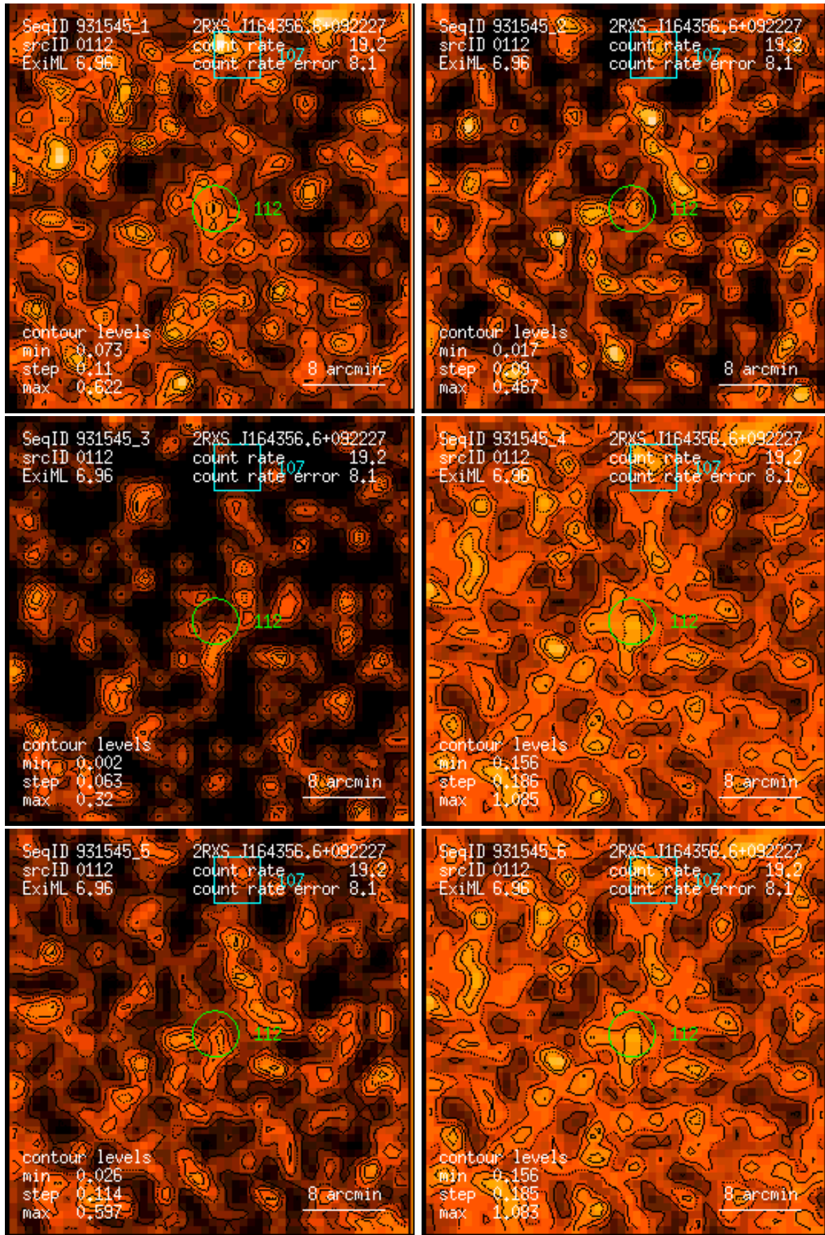
Figure 112: RASS 931545: detection 0112: band rate images, Gaussian filter: (1) PSPC channels 11 – 41, (2) 52 – 90, (3) 91 – 201, (4) 11 – 235, (5) 52 – 201, (6) 11 – 201. Broad band rates in counts/ks. Band rate contour levels in counts/ks/arcmin 2 .
