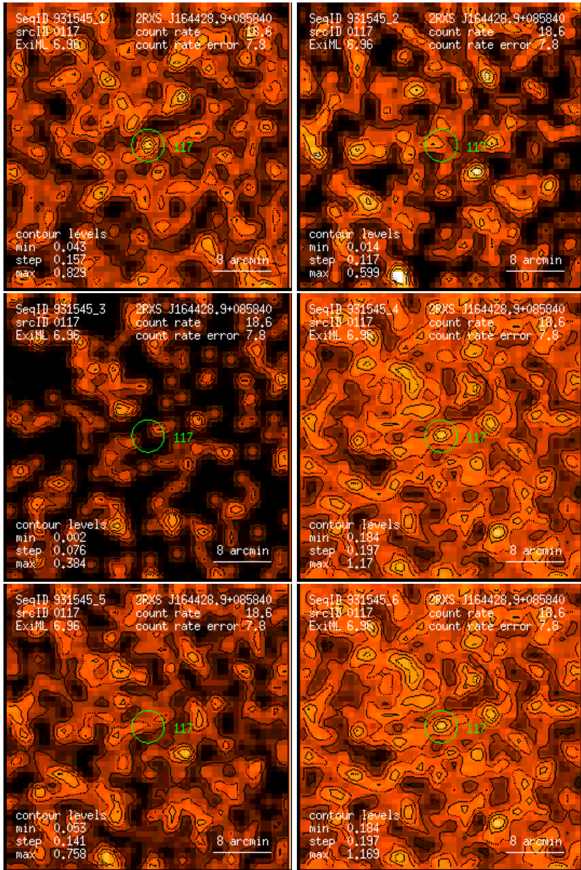
Figure 117: RASS 931545: detection 0117: band rate images, Gaussian filter: (1) PSPC channels 11 – 41, (2) 52 – 90, (3) 91 – 201, (4) 11 – 235, (5) 52 – 201, (6) 11 – 201. Broad band rates in counts/ks. Band rate contour levels in counts/ks/arcmin 2 .
