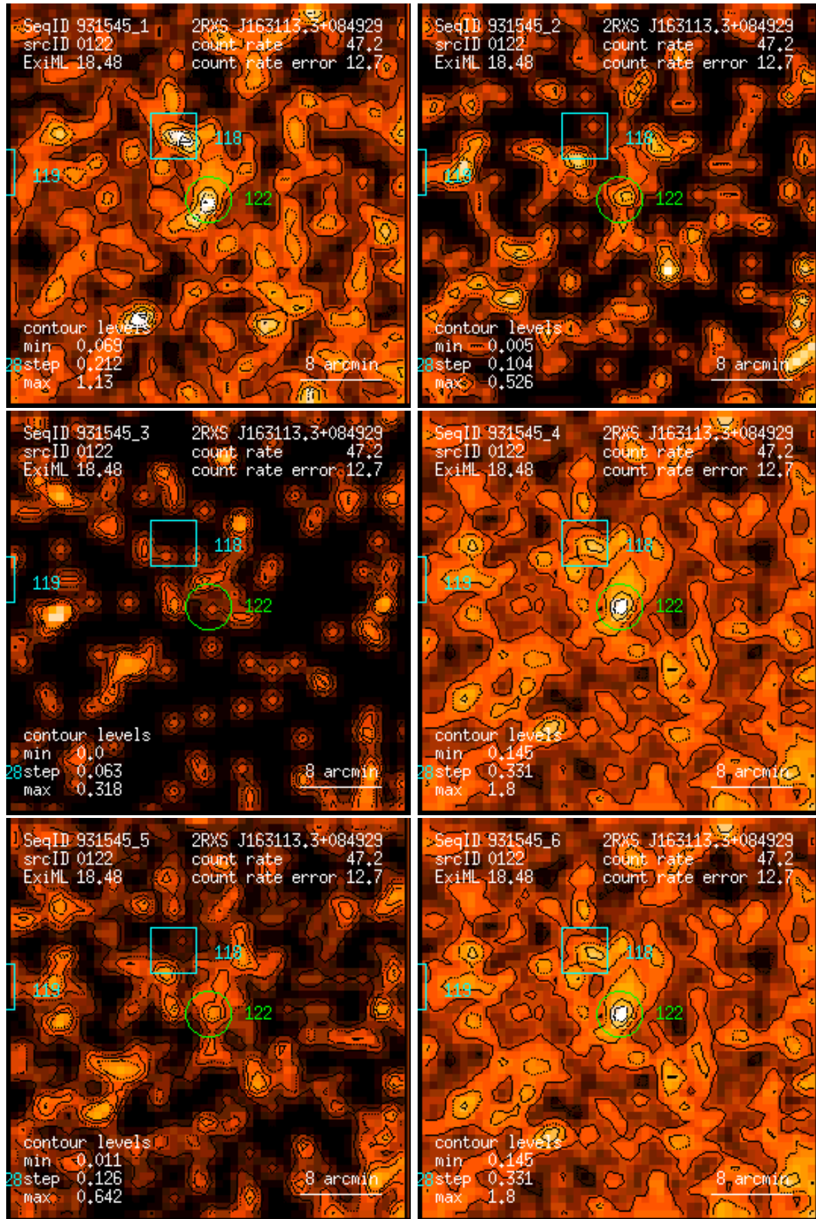
Figure 122: RASS 931545: detection 0122: band rate images, Gaussian filter: (1) PSPC channels 11 – 41, (2) 52 – 90, (3) 91 – 201, (4) 11 – 235, (5) 52 – 201, (6) 11 – 201. Broad band rates in counts/ks. Band rate contour levels in counts/ks/arcmin 2 .
