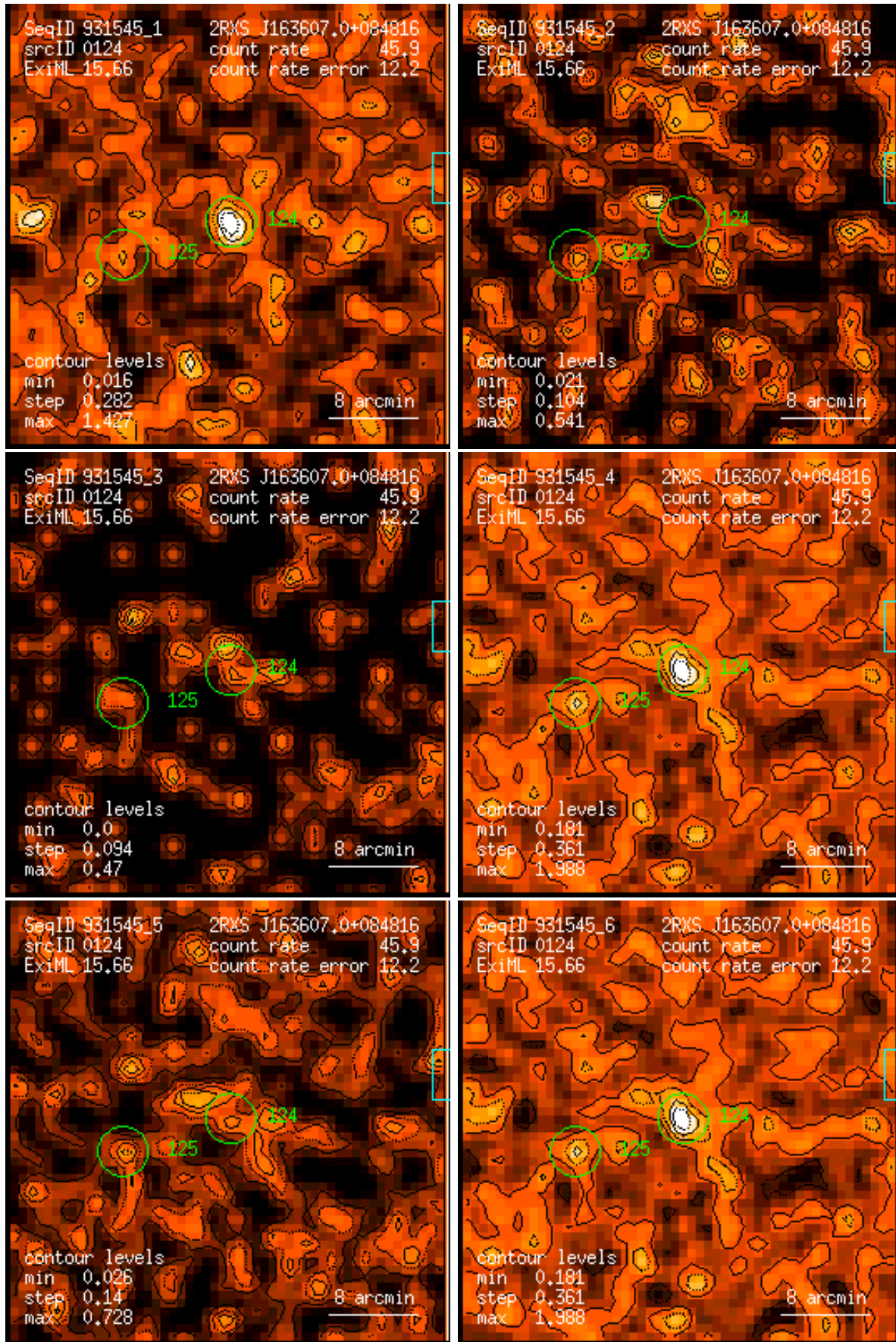
Figure 124: RASS 931545: detection 0124: band rate images, Gaussian filter: (1) PSPC channels 11 – 41, (2) 52 – 90, (3) 91 – 201, (4) 11 – 235, (5) 52 – 201, (6) 11 – 201. Broad band rates in counts/ks. Band rate contour levels in counts/ks/arcmin 2 .
