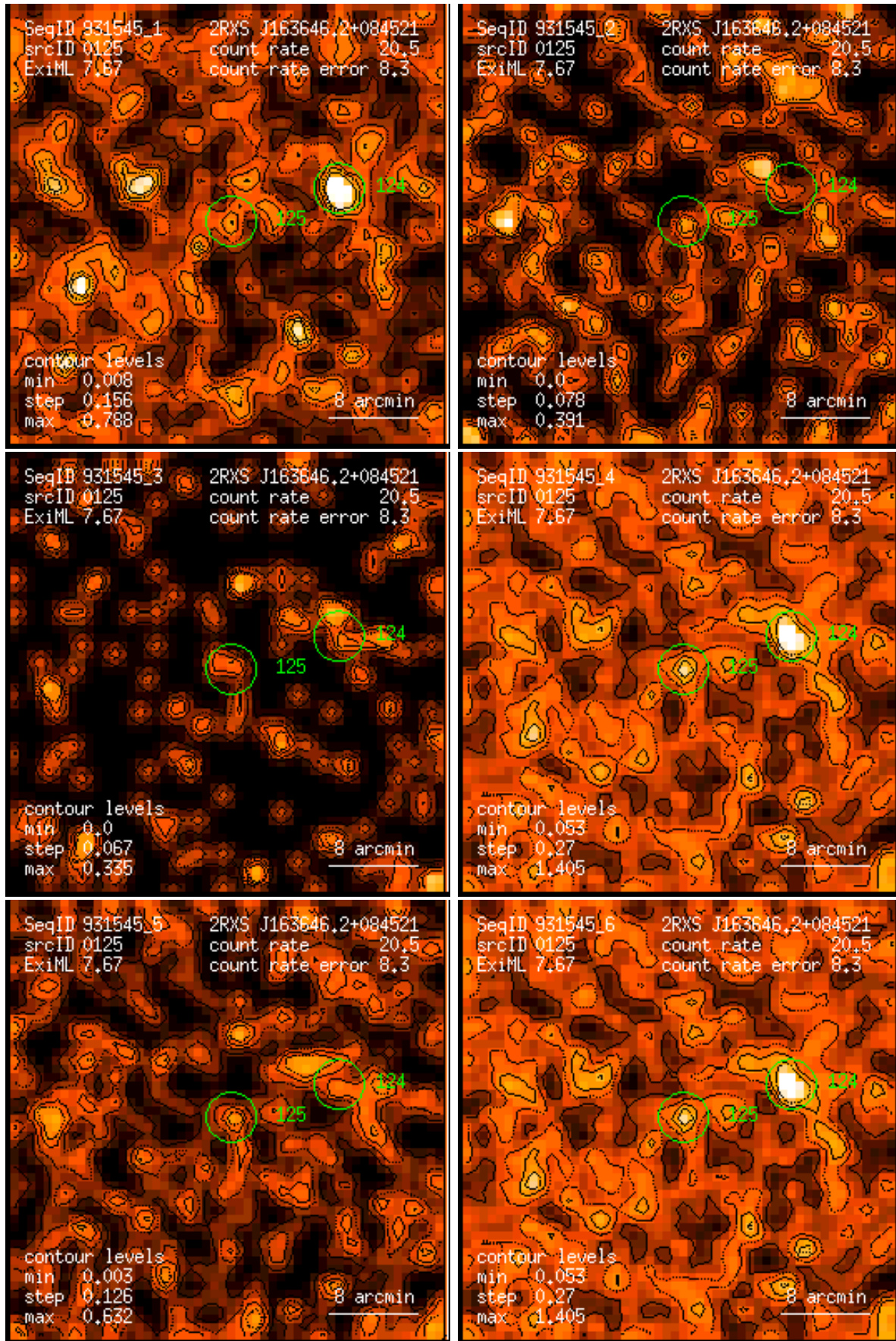
Figure 125: RASS 931545: detection 0125: band rate images, Gaussian filter: (1) PSPC channels 11 – 41, (2) 52 – 90, (3) 91 – 201, (4) 11 – 235, (5) 52 – 201, (6) 11 – 201. Broad band rates in counts/ks. Band rate contour levels in counts/ks/arcmin 2 .
