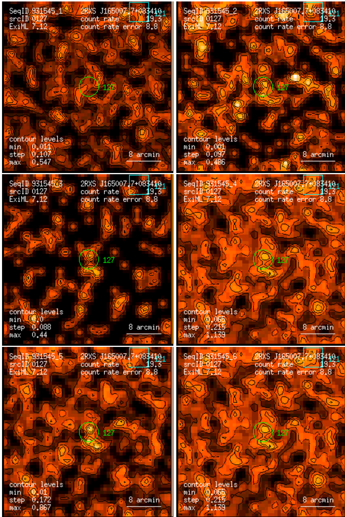
Figure 127: RASS 931545: detection 0127: band rate images, Gaussian filter: (1) PSPC channels 11 – 41, (2) 52 – 90, (3) 91 – 201, (4) 11 – 235, (5) 52 – 201, (6) 11 – 201. Broad band rates in counts/ks. Band rate contour levels in counts/ks/arcmin 2 .
