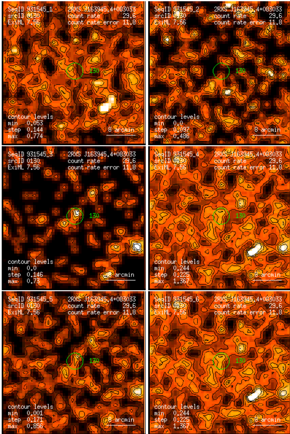
Figure 130: RASS 931545: detection 0130: band rate images, Gaussian filter: (1) PSPC channels 11 – 41, (2) 52 – 90, (3) 91 – 201, (4) 11 – 235, (5) 52 – 201, (6) 11 – 201. Broad band rates in counts/ks. Band rate contour levels in counts/ks/arcmin 2 .
