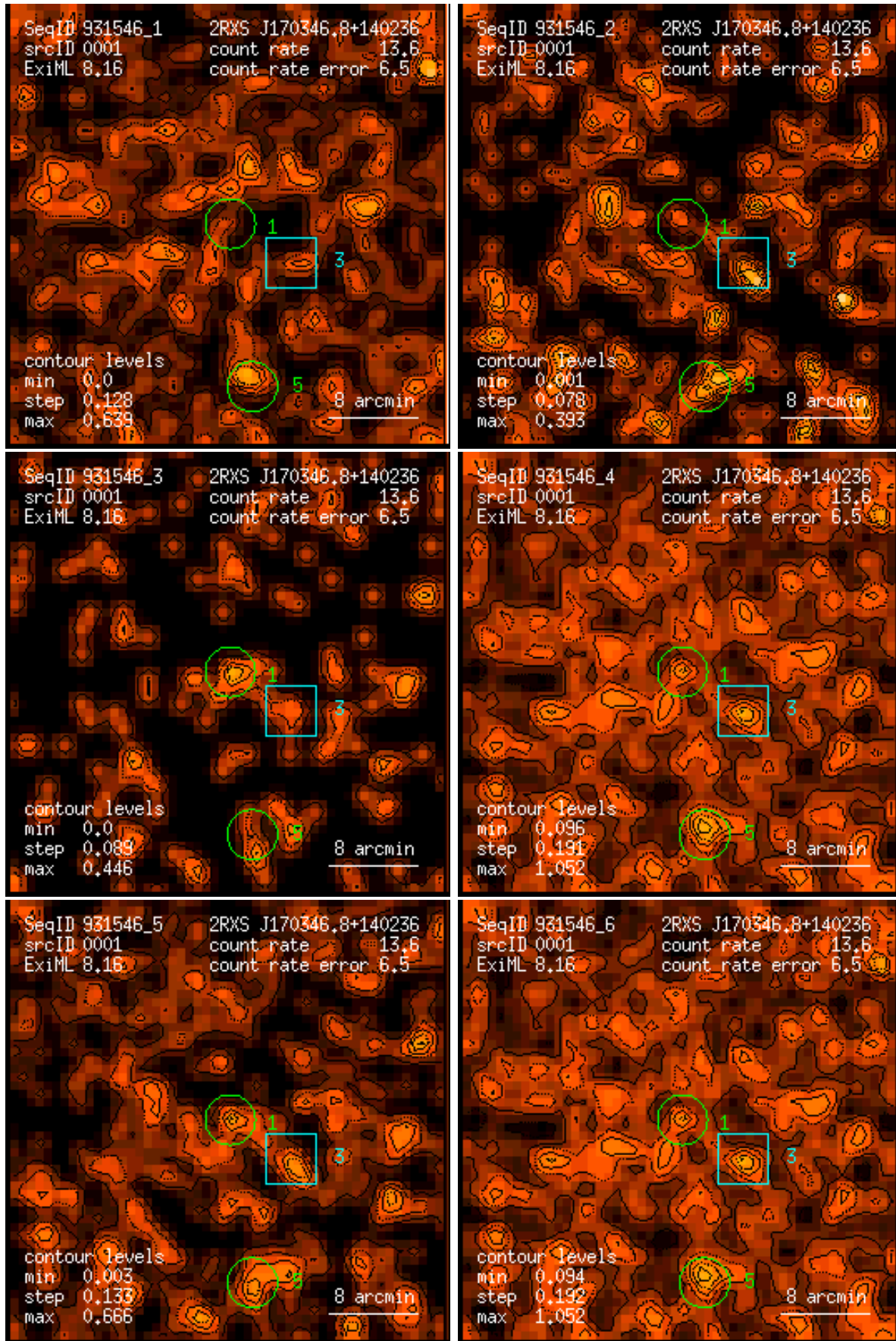
Figure 1: RASS 931546: detection 0001: band rate images, Gaussian filter: (1) PSPC channels 11 – 41, (2) 52 – 90, (3) 91 – 201, (4) 11 – 235, (5) 52 – 201, (6) 11 – 201. Broad band rates in counts/ks. Band rate contour levels in counts/ks/arcmin 2 .
