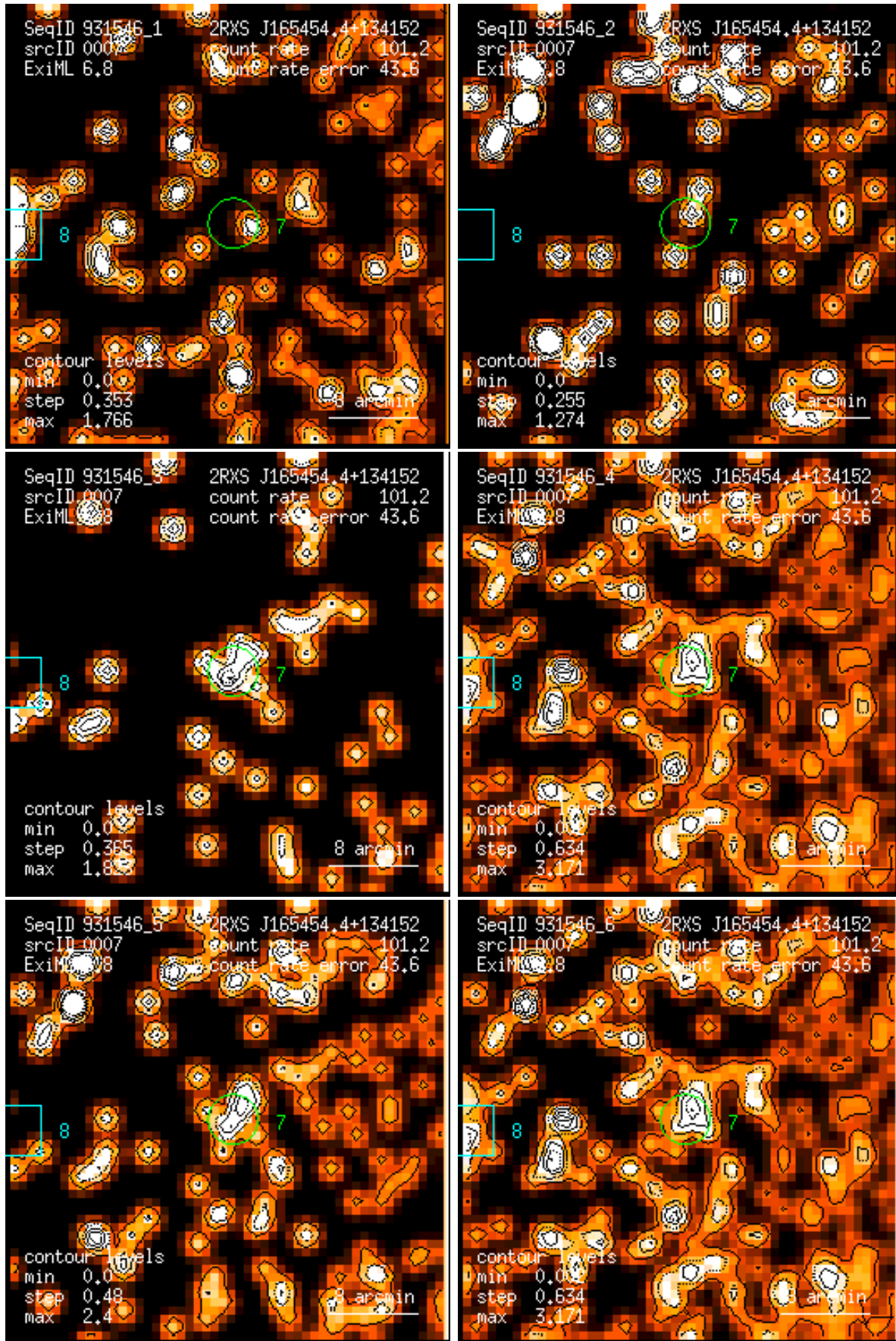
Figure 7: RASS 931546: detection 0007: band rate images, Gaussian filter: (1) PSPC channels 11 – 41, (2) 52 – 90, (3) 91 – 201, (4) 11 – 235, (5) 52 – 201, (6) 11 – 201. Broad band rates in counts/ks. Band rate contour levels in counts/ks/arcmin 2 .
