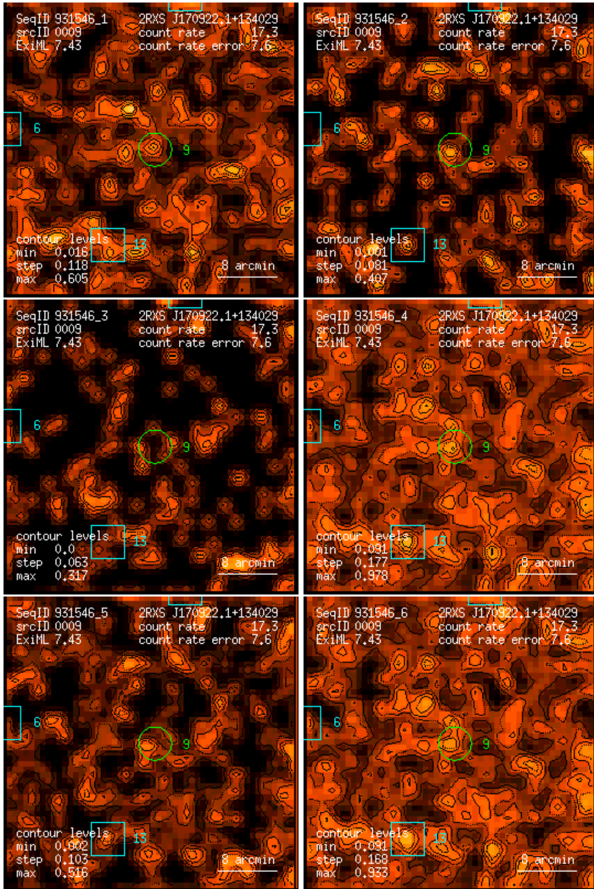
Figure 9: RASS 931546: detection 0009: band rate images, Gaussian filter: (1) PSPC channels 11 – 41, (2) 52 – 90, (3) 91 – 201, (4) 11 – 235, (5) 52 – 201, (6) 11 – 201. Broad band rates in counts/ks. Band rate contour levels in counts/ks/arcmin 2 .
