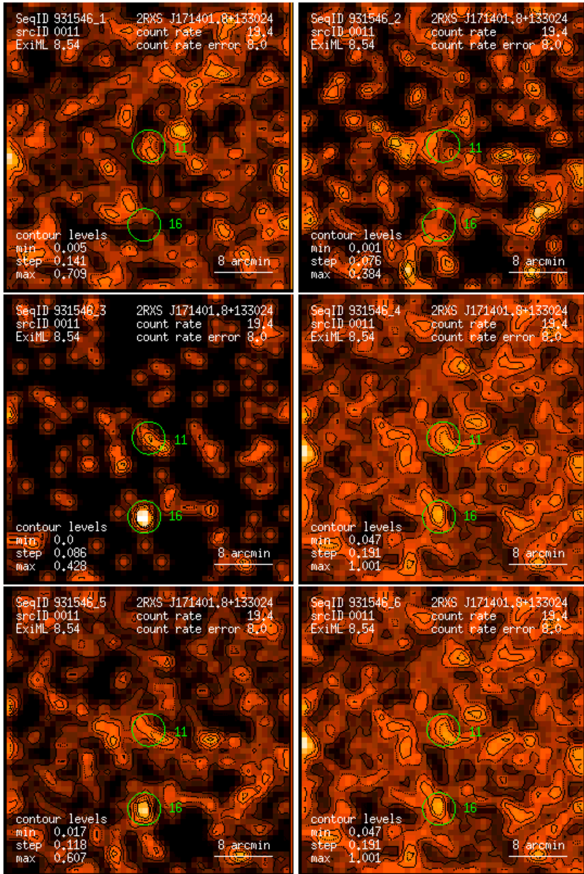
Figure 11: RASS 931546: detection 0011: band rate images, Gaussian filter: (1) PSPC channels 11 – 41, (2) 52 – 90, (3) 91 – 201, (4) 11 – 235, (5) 52 – 201, (6) 11 – 201. Broad band rates in counts/ks. Band rate contour levels in counts/ks/arcmin 2 .
