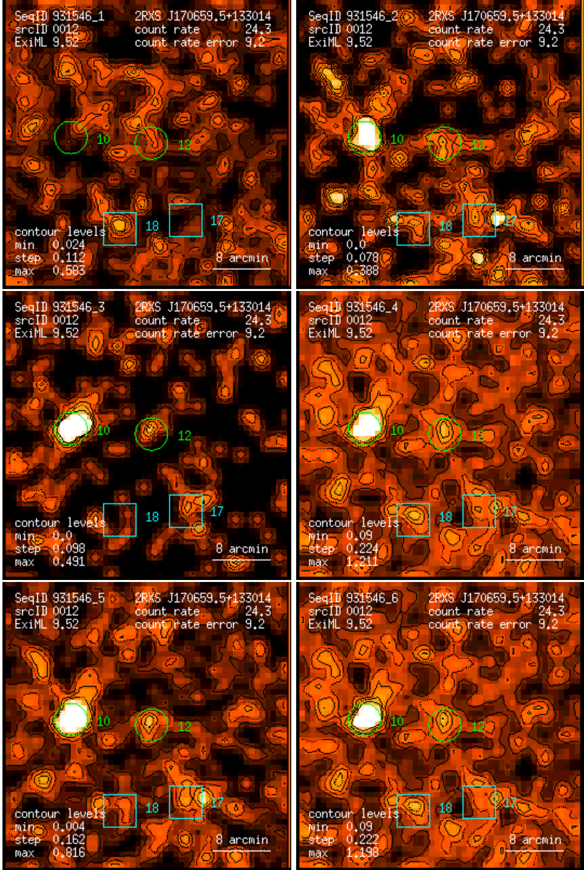
Figure 12: RASS 931546: detection 0012: band rate images, Gaussian filter: (1) PSPC channels 11 – 41, (2) 52 – 90, (3) 91 – 201, (4) 11 – 235, (5) 52 – 201, (6) 11 – 201. Broad band rates in counts/ks. Band rate contour levels in counts/ks/arcmin 2 .
