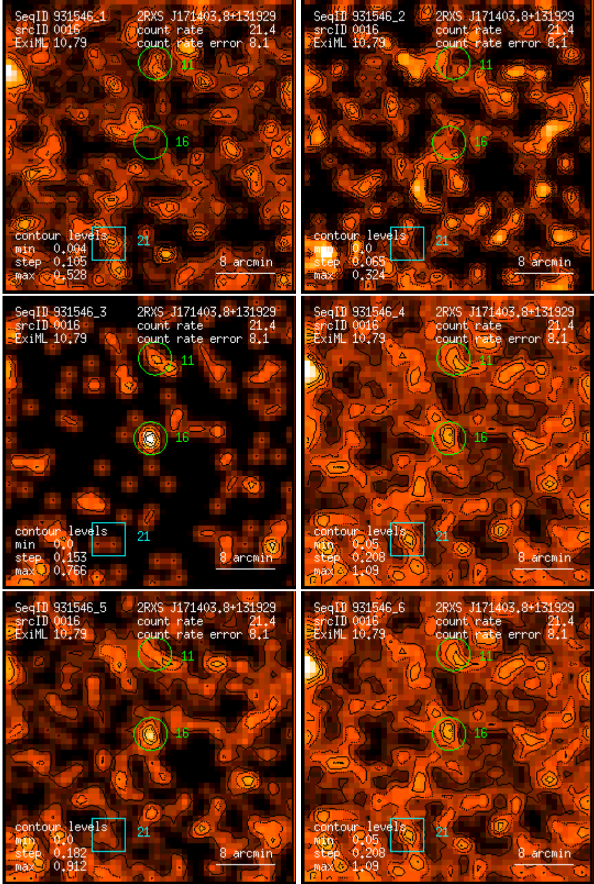
Figure 16: RASS 931546: detection 0016: band rate images, Gaussian filter: (1) PSPC channels 11 – 41, (2) 52 – 90, (3) 91 – 201, (4) 11 – 235, (5) 52 – 201, (6) 11 – 201. Broad band rates in counts/ks. Band rate contour levels in counts/ks/arcmin 2 .
