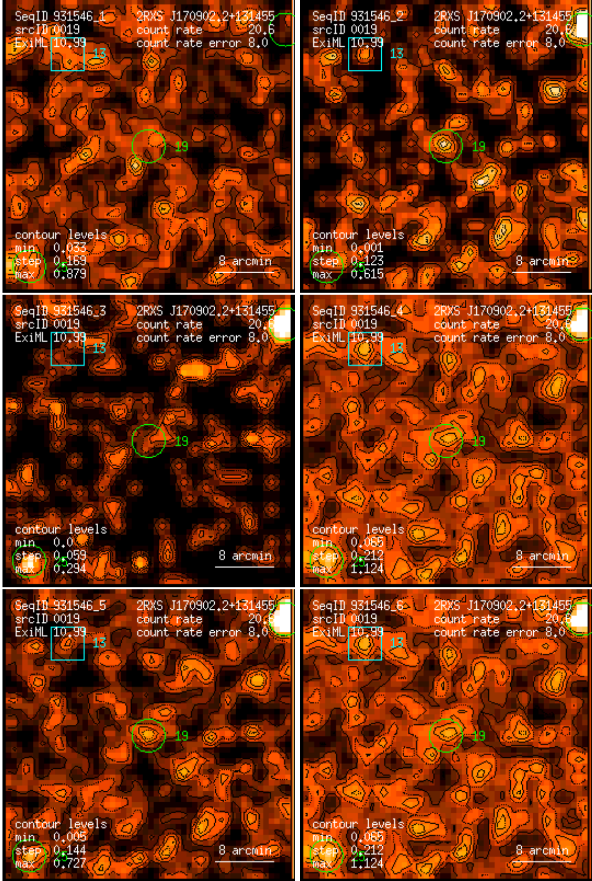
Figure 19: RASS 931546: detection 0019: band rate images, Gaussian filter: (1) PSPC channels 11 – 41, (2) 52 – 90, (3) 91 – 201, (4) 11 – 235, (5) 52 – 201, (6) 11 – 201. Broad band rates in counts/ks. Band rate contour levels in counts/ks/arcmin 2 .
