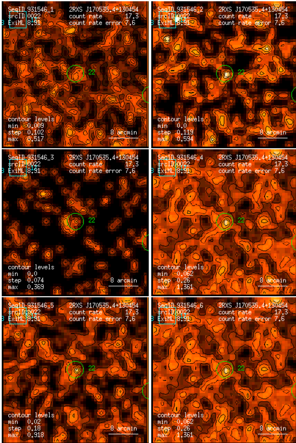
Figure 22: RASS 931546: detection 0022: band rate images, Gaussian filter: (1) PSPC channels 11 – 41, (2) 52 – 90, (3) 91 – 201, (4) 11 – 235, (5) 52 – 201, (6) 11 – 201. Broad band rates in counts/ks. Band rate contour levels in counts/ks/arcmin 2 .
