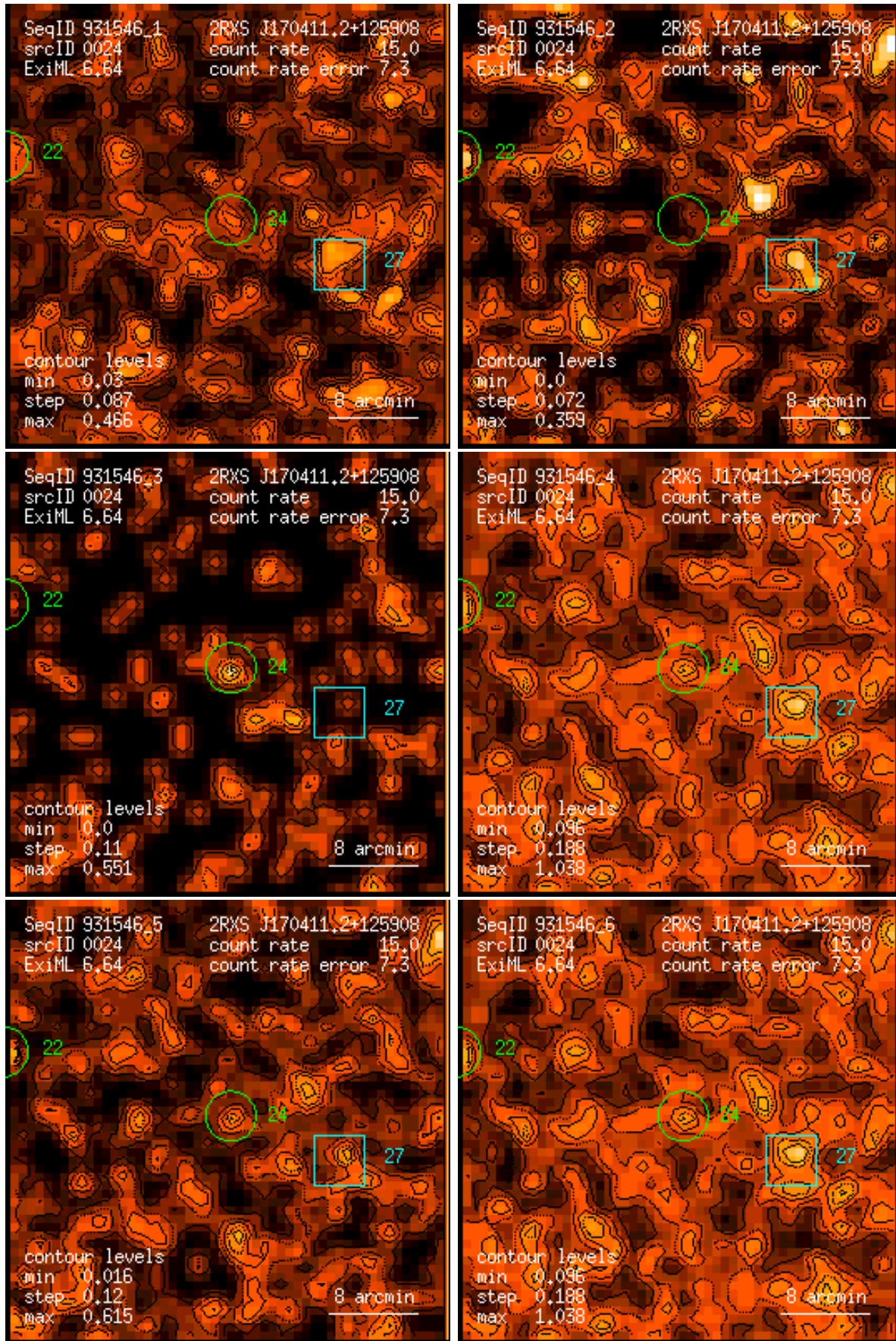
Figure 24: RASS 931546: detection 0024: band rate images, Gaussian filter: (1) PSPC channels 11 – 41, (2) 52 – 90, (3) 91 – 201, (4) 11 – 235, (5) 52 – 201, (6) 11 – 201. Broad band rates in counts/ks. Band rate contour levels in counts/ks/arcmin 2 .
