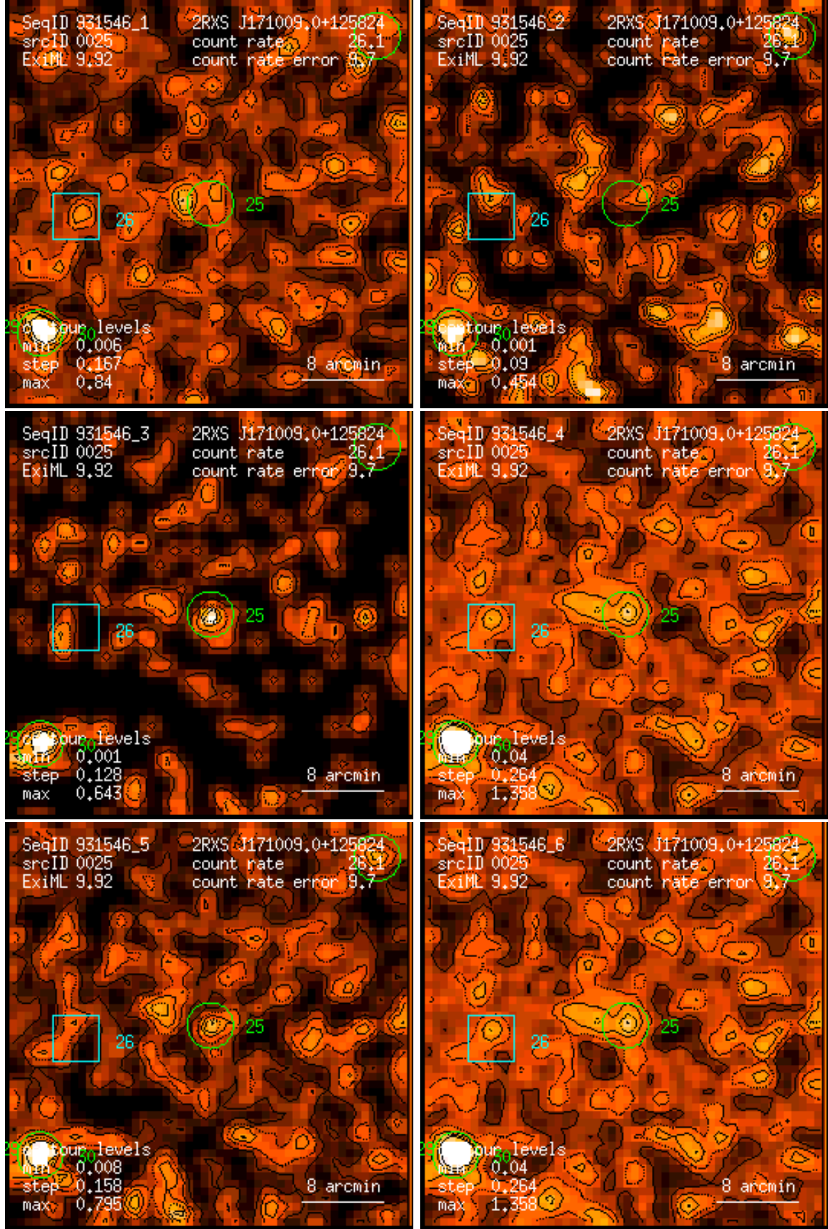
Figure 25: RASS 931546: detection 0025: band rate images, Gaussian filter: (1) PSPC channels 11 – 41, (2) 52 – 90, (3) 91 – 201, (4) 11 – 235, (5) 52 – 201, (6) 11 – 201. Broad band rates in counts/ks. Band rate contour levels in counts/ks/arcmin 2 .
