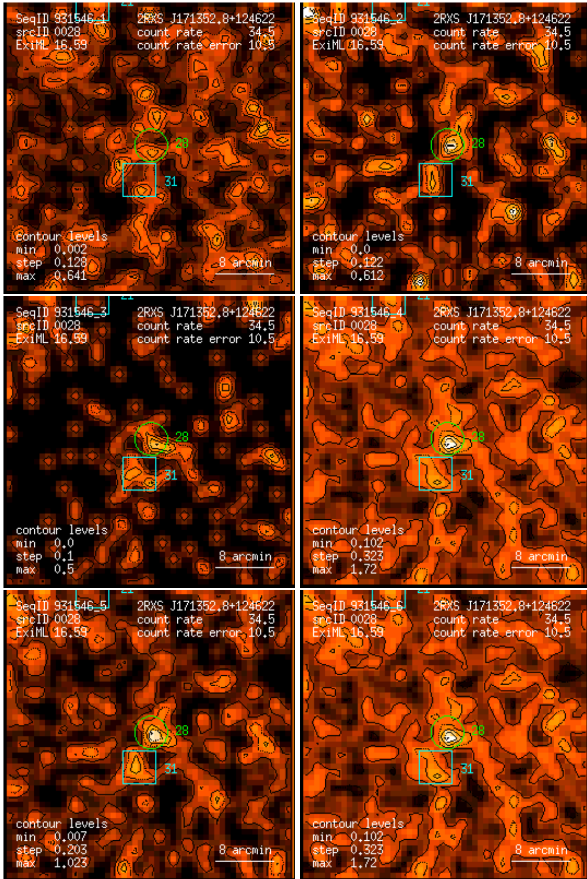
Figure 28: RASS 931546: detection 0028: band rate images, Gaussian filter: (1) PSPC channels 11 – 41, (2) 52 – 90, (3) 91 – 201, (4) 11 – 235, (5) 52 – 201, (6) 11 – 201. Broad band rates in counts/ks. Band rate contour levels in counts/ks/arcmin 2 .
